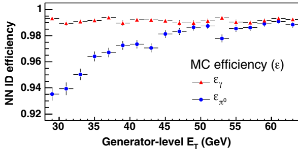
FIG. 1 (color online). Comparison of the \gamma and \pi^0 NN selection efficiencies, obtained using the special-purpose MC event generator. The efficiency is shown as a function of the generator-level E_T .
