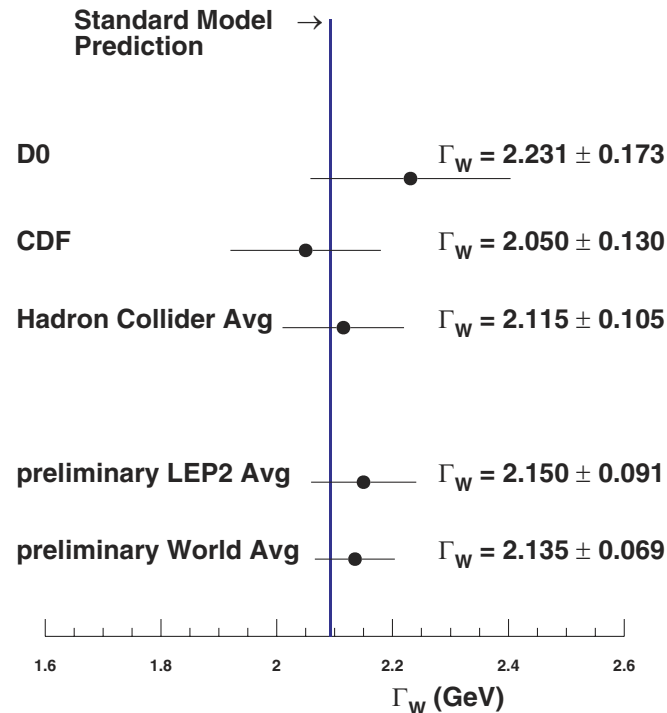
FIG. 2 (color online). Direct measurements of the W boson width compared with the SM prediction [23].
