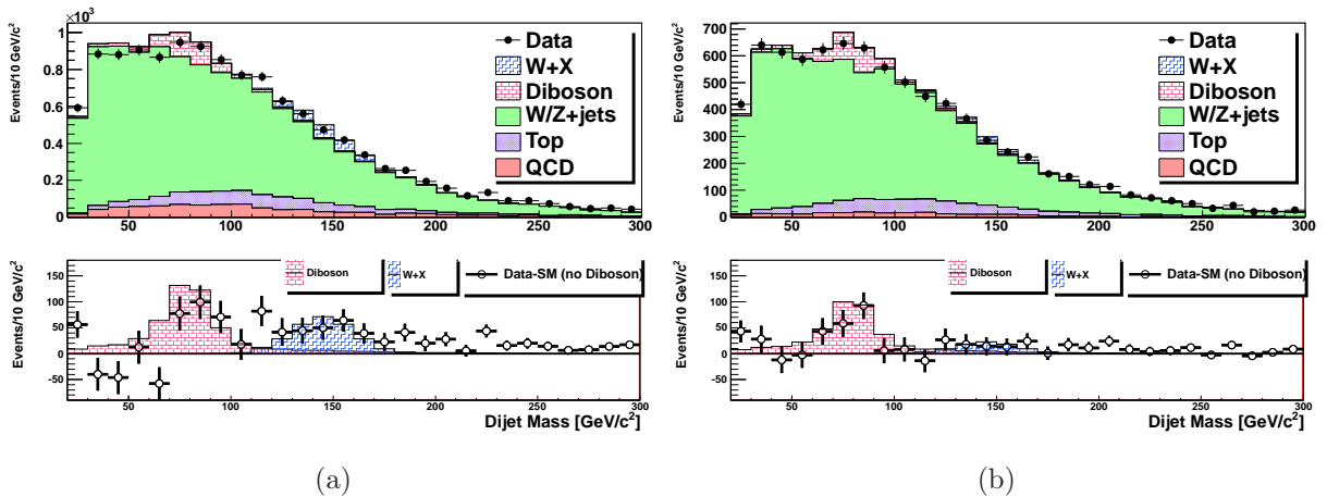
FIG. 8. Same distribution as in Fig. 7, shown separately for the electron (a) and muon (b) samples.
