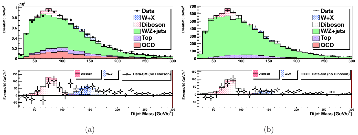
FIG. 11. Same distribution as in Fig. 10, shown separately for the electron (a) and muon (b) samples.
