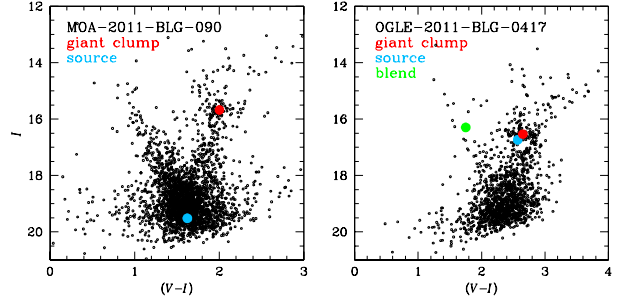
FIG. 4.— OGLE color-magnitude diagrams of stars in the fields where the lensing events MOA-2011-BLG-090 (left panel) and OGLE-2011-BLG-0417 (right panel) occurred. The red and blue dots represent the centroid of the giant clump and the location of the source star for each event, respectively. For OGLE-2011-BLG-0417, we also mark the position of the blended star.
