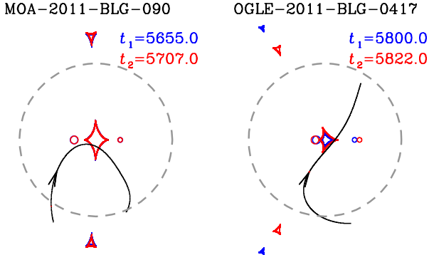
FIG. 3.— The caustic geometries and source trajectories of the best-fit models for MOA-2011-BLG-090 (left panel) and OGLE-2011-BLG-0417 (right panel). The small closed figures composed of concave curves represent the caustics. The small open circles represent the lens positions. We note that the lens positions and the resulting caustic vary in time due to the orbital motion of the lens. We mark 2 sets of lens positions and caustics at 2 different times of t_1 and t_2 . We also note that the source trajectory, the curve with an arrow, is curved due to the combination of the parallax and orbital effects. The source trajectory is presented so that the binary axis is set along the horizontal axis. The dashed circles represent the Einstein rings corresponding to the total mass of the binary lenses.
