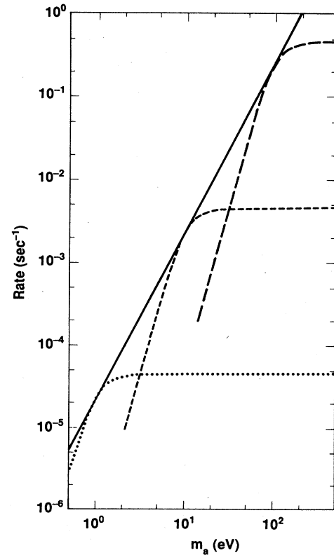
FIG. 7. Total rate of axion-photon conversion in the absorption type detector: dotted line, gas mixture and pressure chosen to maximize the count rate for m_a \approx 1 eV; dashed line, optimized for m_a \approx 10 eV; long-dashed line, for m_a \approx 100 eV; solid line, the envelope curve for m_a \approx m_\Gamma , also plotted in Fig. 6.
