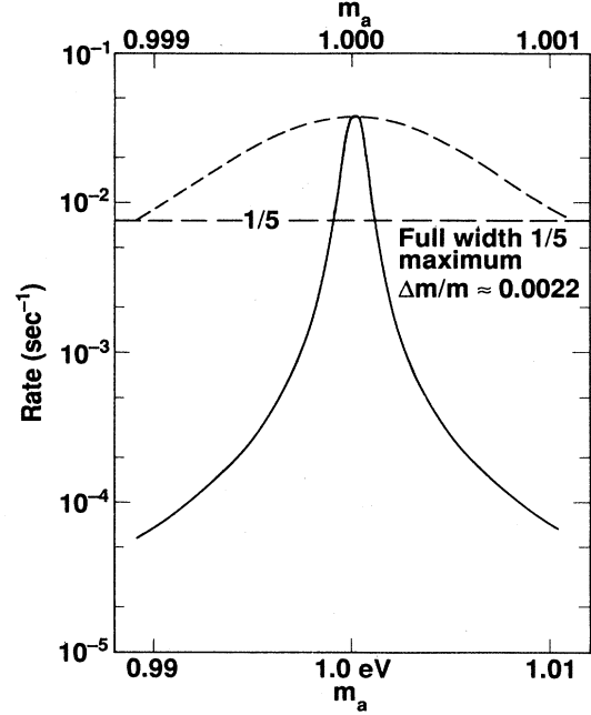
FIG. 5. Conversion rate as a function of m_a for the detector shown in Fig. 4, with D = 4 m, S = 3 m, and B = 3 T. The dispersion gas density is chosen such that m_\gamma = 1.000 eV, and thus is optimized for conversion of axions with m_a = 1.000 eV. The dashed line is a blow-up of the solid line; the corresponding scale is on the upper horizontal axis.
