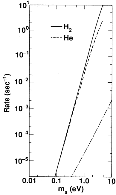
FIG. 6. Total rate of axion-photon conversion in the dispersion-matching detector as a function of the axion mass m_a . As in Fig. 5, the relationship between m_a and the axion-photon coupling M is given by Eq. (4) and the GUT value E/N=8/3 is used. The density of the dispersion gas is assumed to be readjusted to the optimal value for each value of m_a . At the largest values of m_a , corresponding to the highest gas densities, the rate with He as a dispersion gas (dashed line) is lower than that for H_2 (solid line) because of the increased importance of absorption in the higher- Z medium. The dashed-dotted line indicates the conversion rate in an absorption gas detector with m_a = m_\Gamma for comparison. Although the sensitivity is much lower, it is sensitive to a wide range of axion masses simultaneously.
