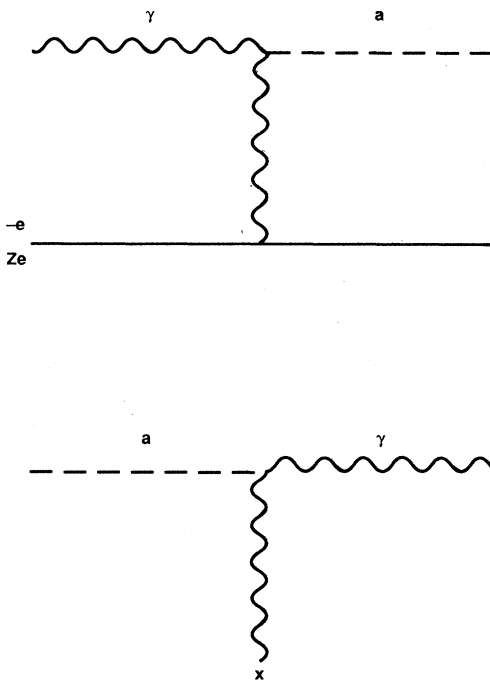
FIG. 1. Feynman diagram for the Primakoff production of axions by the interaction of a photon with an electron or nucleus (top), and (bottom) axion-photon conversion in the electric or magnetic field of an external source denoted by a cross (X).
