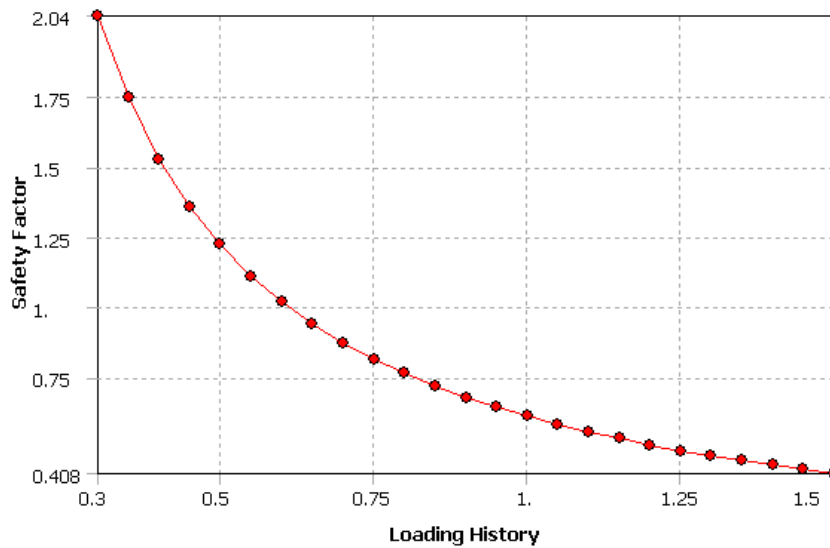
Fig 4.26: Fatigue Sensitivity to Safety Factor Plot for Zero Based Loading
