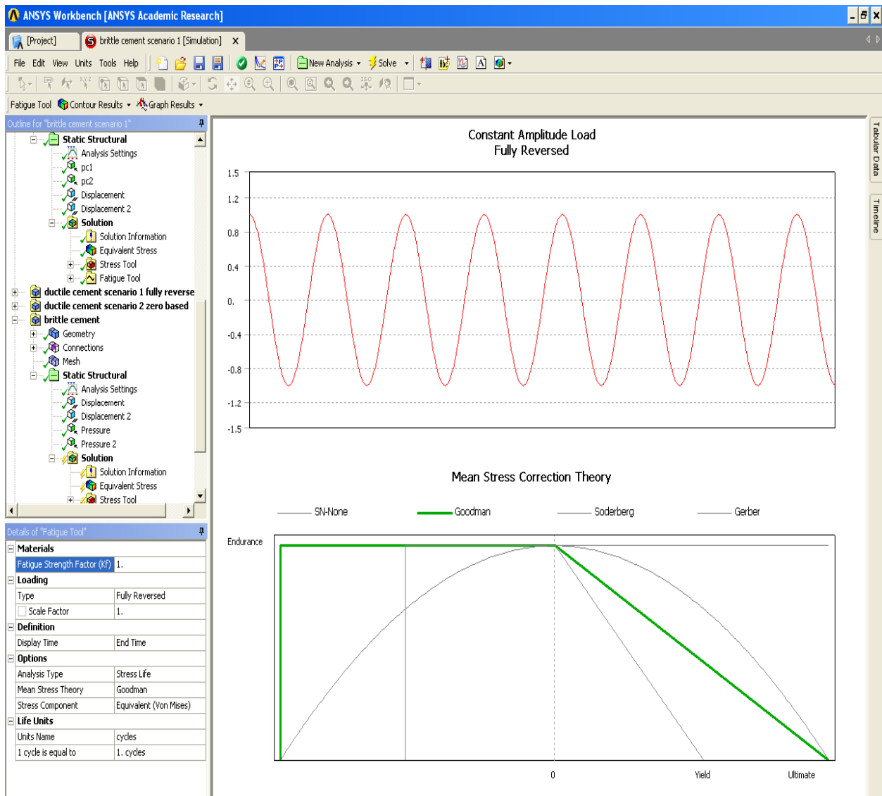
Fig 3.14: Fully Reversed Loading, Goodman's Diagram and Fatigue Options
