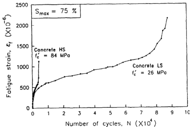
Fig 1.2: Comparison of Fatigue Strain for High and Low Strength Cements [2]
