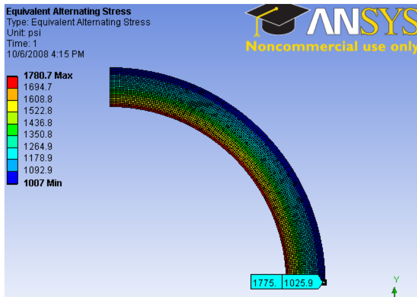
Fig 4.39: Alternating Stress for Cement System 1 under Zero Based Cyclic Loading
