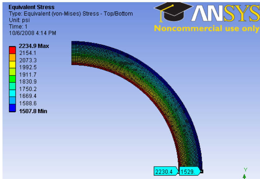
Fig 4.38: Equivalent Stress for Cement System 1 under Static Loading
