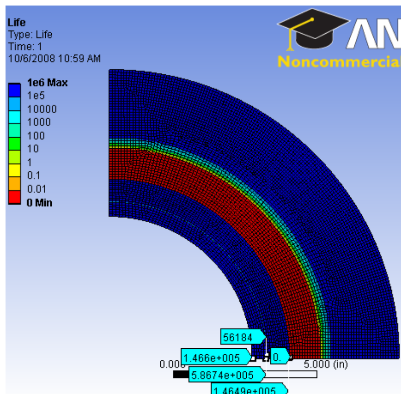
Fig 4.24: Life Cycle for Zero Based Loading
