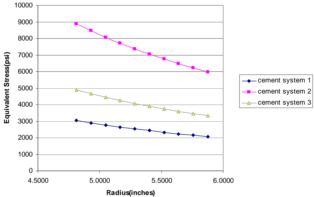
Fig 4.3: Equivalent Stress in Three Cement Systems with p_i=15000 psi and p_f=1000 psi
