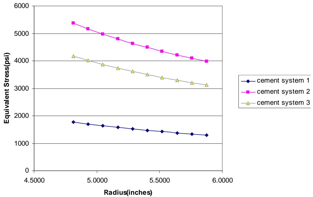
Fig 4.19: Equivalent Stress with p_i=4000 psi, p_f=10000 psi and \Delta T =150^\circ\text{F}
