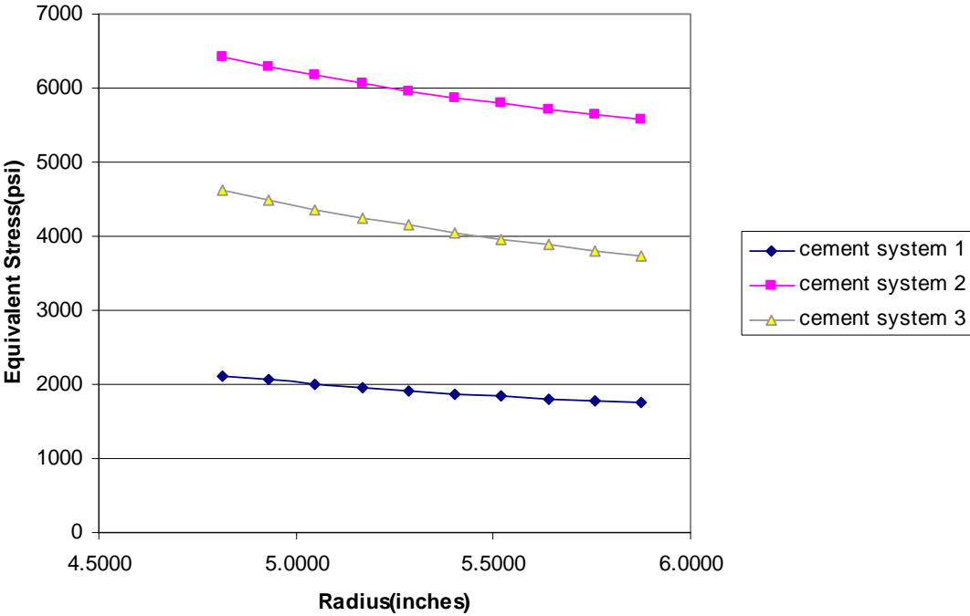
Fig 4.10: Equivalent Stress in Three Cement Systems with p_i=4000 psi and p_f=10000 psi
