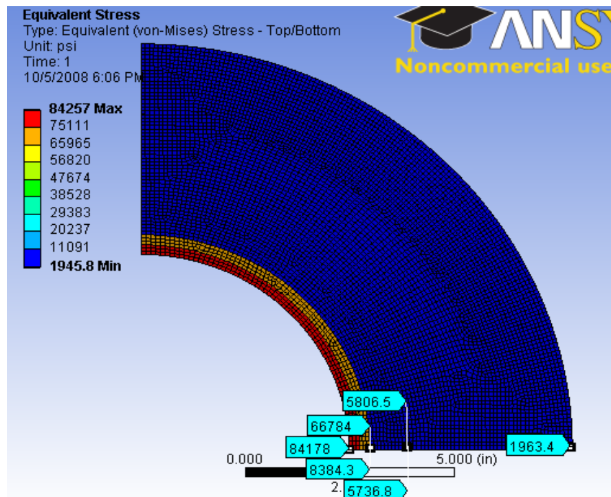
Fig 4.1: Equivalent Stress with Formation E=3 \times 10^6 psi and \nu=0.42 for Scenario 1
