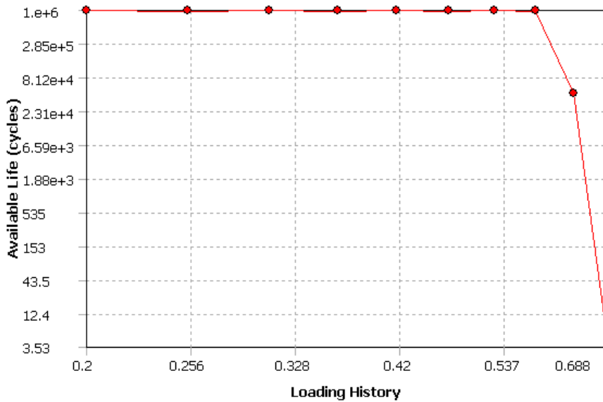
Fig 4.25: Fatigue Sensitivity to Life Plot for Zero Based Loading
