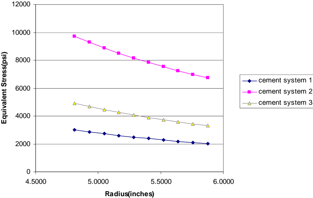
Fig 4.13: Equivalent Stress with p_i=15000 psi, p_f=1000 psi and \Delta T =150^\circ\text{F}
