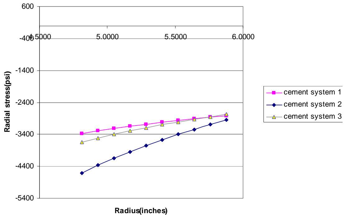
Fig 4.9: Radial Stress in Three Cement Systems with p_i=15000 psi and p_f=0 psi
