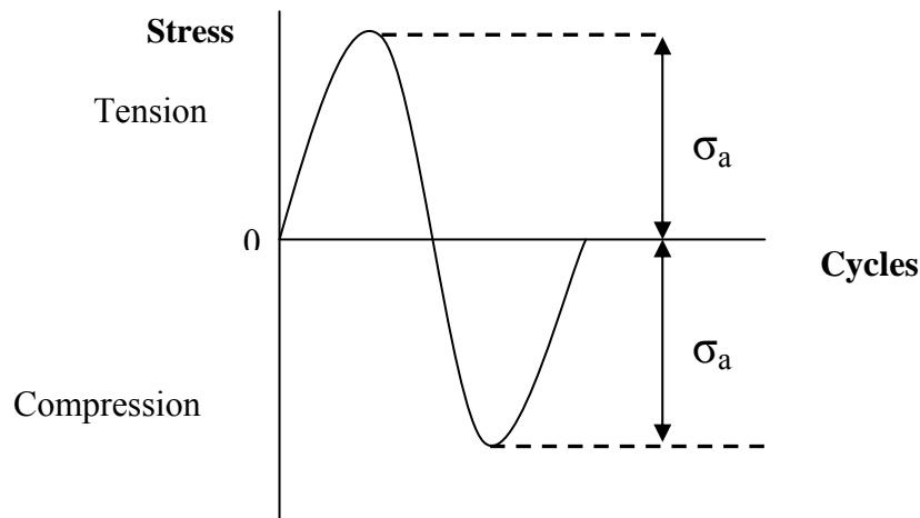
Fig 1.1: Fluctuating Tensile and Compressive Cyclic Stress
