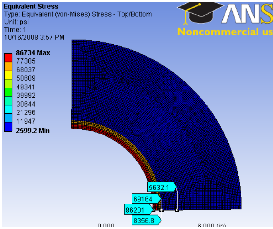
Fig 3.8: Equivalent Stress for Casing –Cement –Formation Model with Meshing
