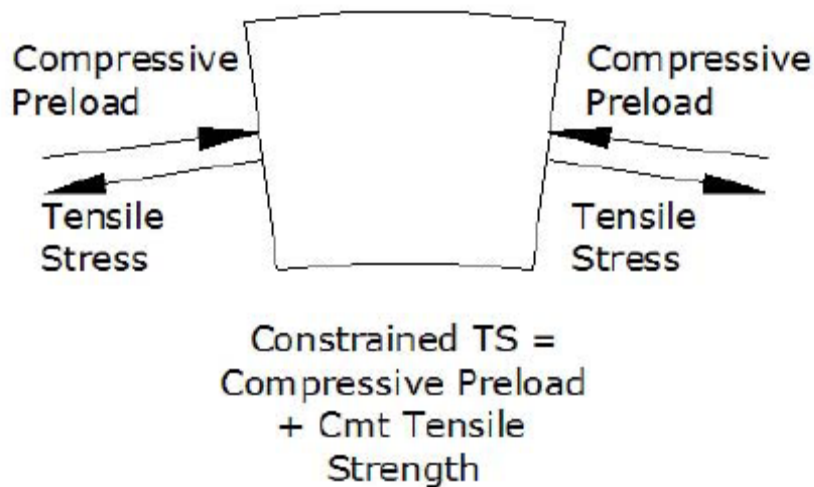
Fig 2.1: Stresses That Act on a Pre-Stressed Cement System [11]
