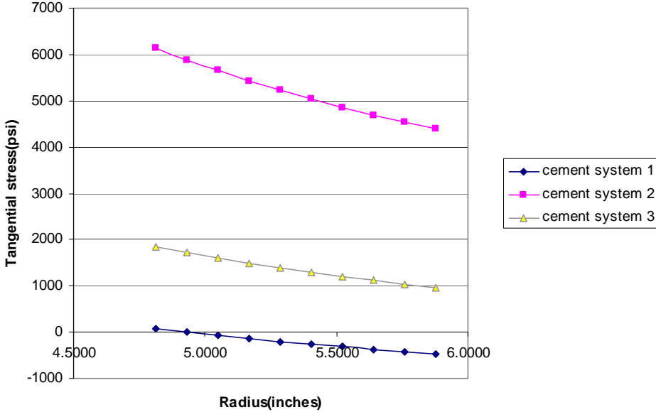
Fig 4.17: Tangential Stress with p_i=15000 psi, p_f= 0 psi and \Delta T =150^\circ\text{F}
