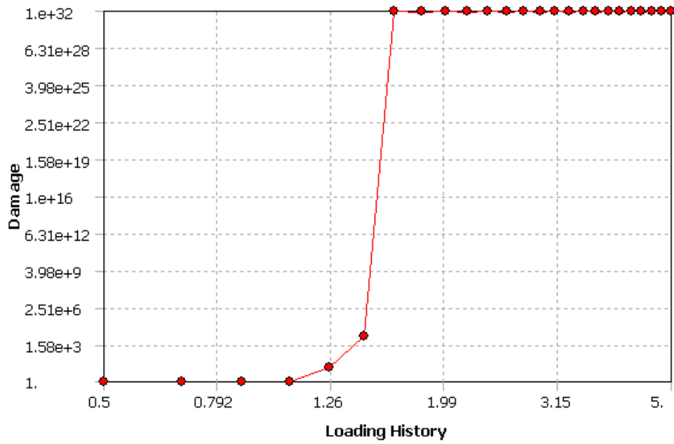
Fig 4.43: Fatigue Sensitivity to Damage for Zero Based Cyclic Loading with Cement 1
