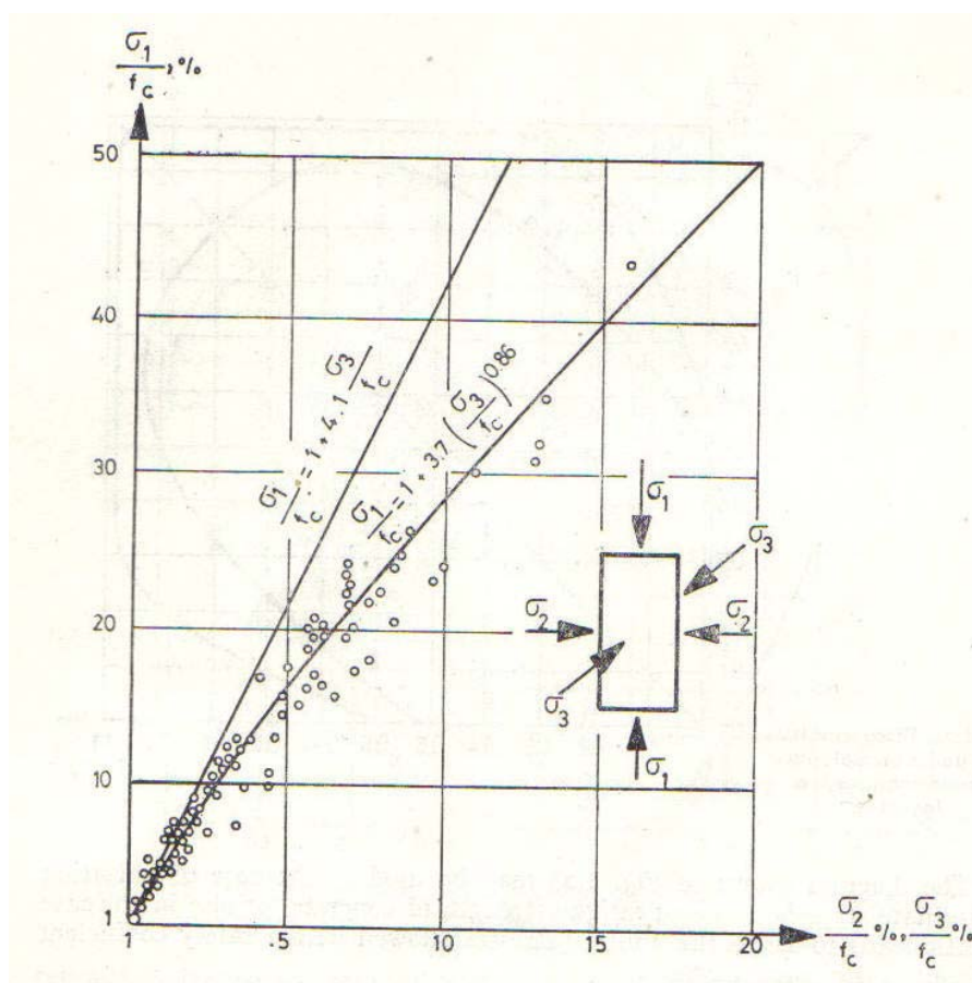
Fig 3.3: Concrete Failure Criterion under Triaxial Compressive Stresses [24]
