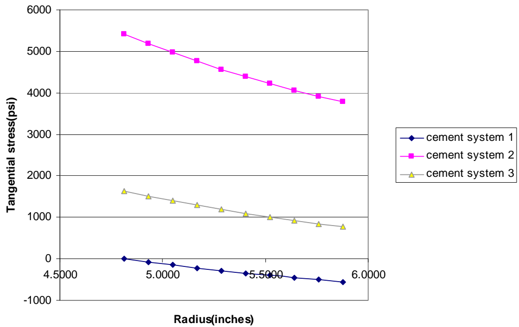
Fig 4.8: Tangential Stress in Three Cement Systems with p_i=15000 psi and p_f=0 psi
