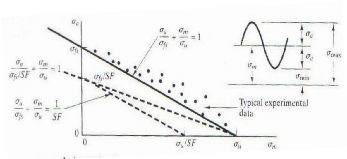
Fig 3.12: Goodman Diagram for Brittle and Ductile Materials [1]
