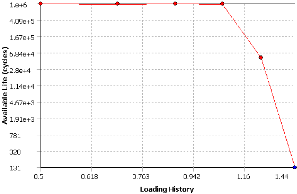
Fig 4.41: Fatigue Sensitivity to Life for Zero Based Cyclic Loading with Cement 1
