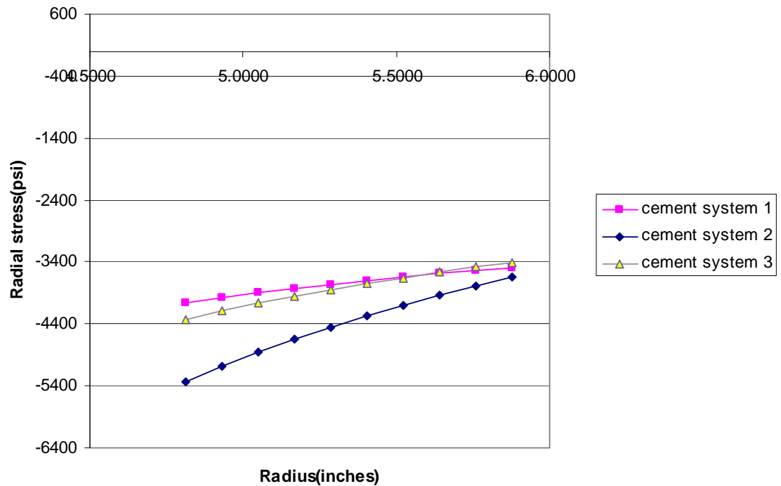
Fig 4.5: Radial Stress in Three Cement Systems with p_i=15000 psi and p_f=1000 psi
