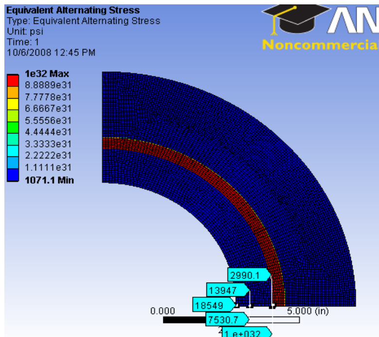
Fig 4.29: Alternating Stress for Zero Based Loading with Formation Property: E=1 \times 10^6 , \nu=0.3
