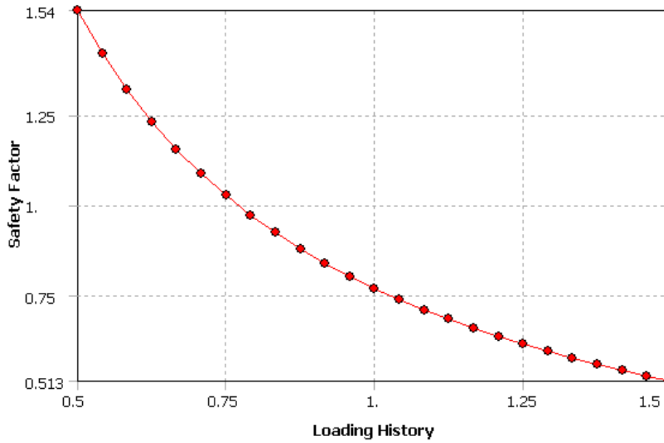
Fig 4.37: Fatigue Sensitivity to Safety Factor plot for a Zero Based Cyclic Loading with Cement 2
