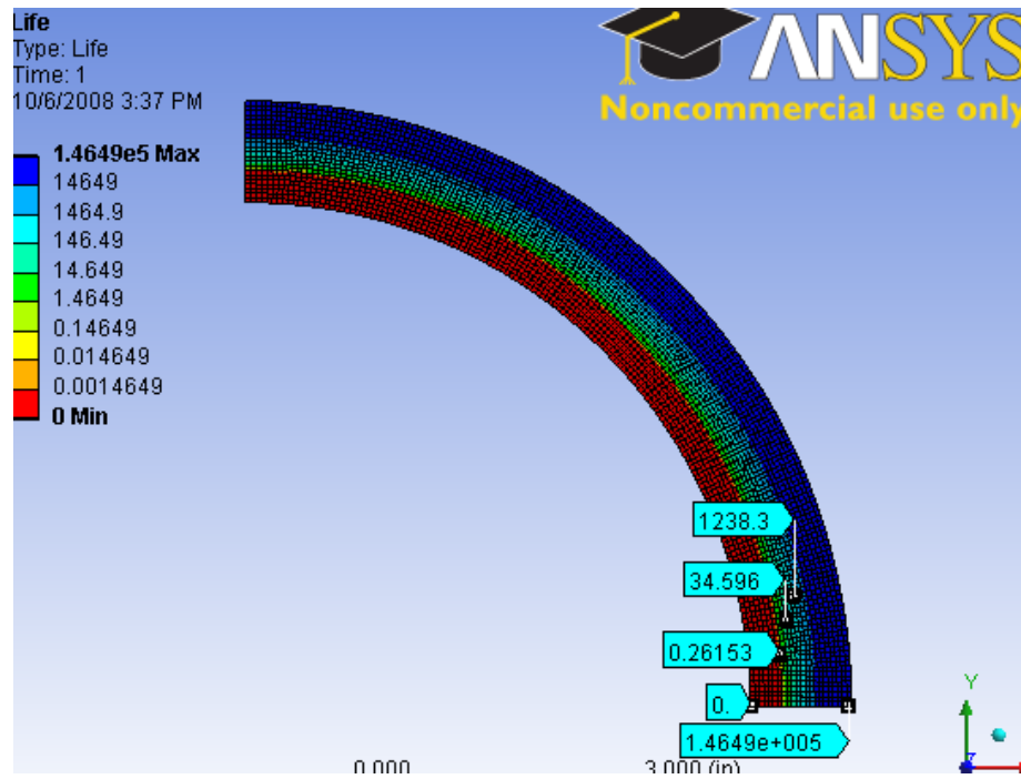
Fig 4.34: Life Cycle for Cement System 2 under a Zero Based Cyclic Loading
