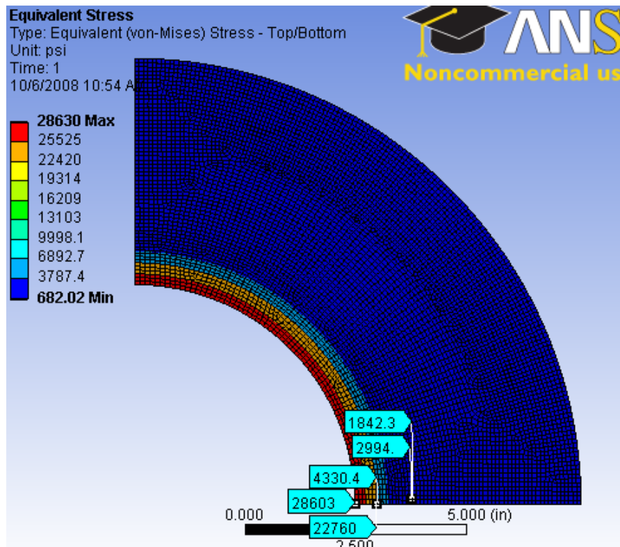
Fig 4.22: Equivalent Stress for Static Loading with Formation E=1 \times 10^6 psi and \nu=0.42
