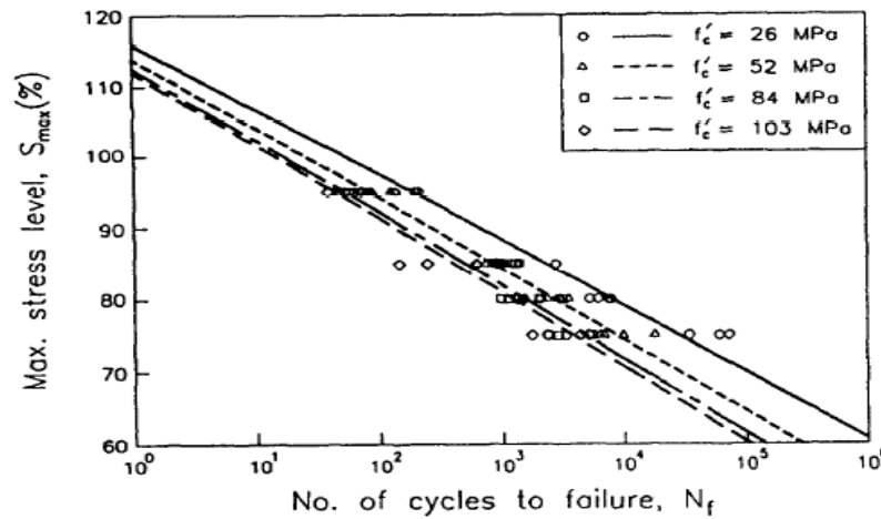
Fig 1.3: Comparison of Max Stress Levels to Number of Cycles for Different Cement Strengths [2]
