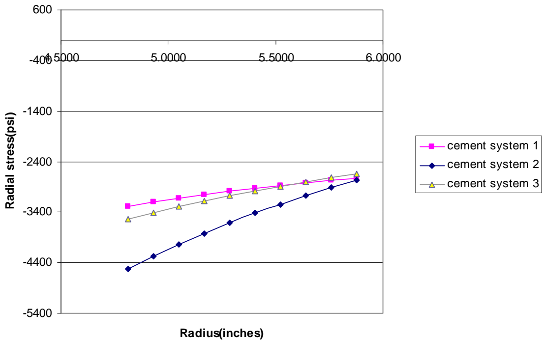
Fig 4.18: Radial Stress with p_i=15000 psi, p_f= 0 psi and \Delta T =150^\circ\text{F}
