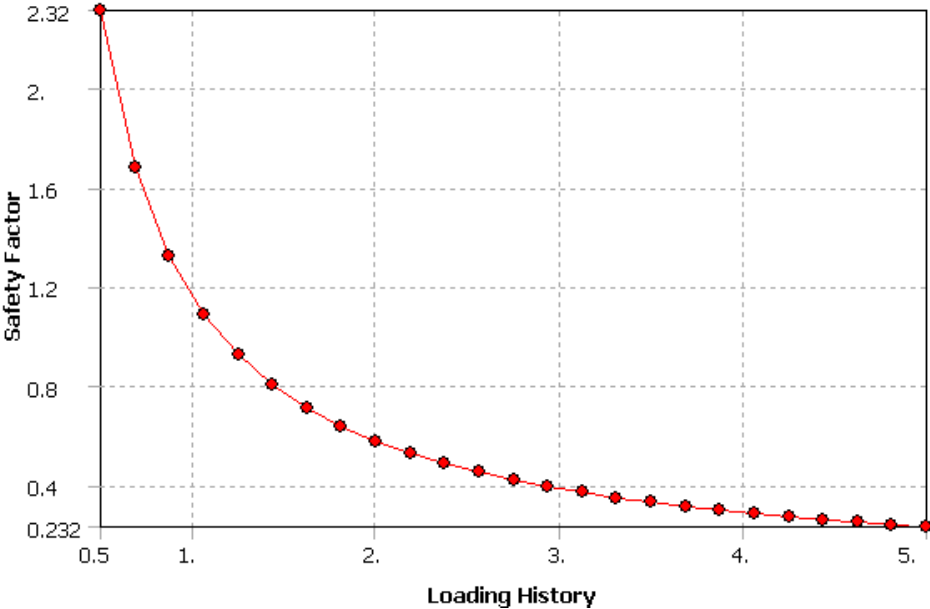
Fig 4.42: Fatigue Sensitivity to Safety Factor for Zero Based Cyclic Loading with Cement
