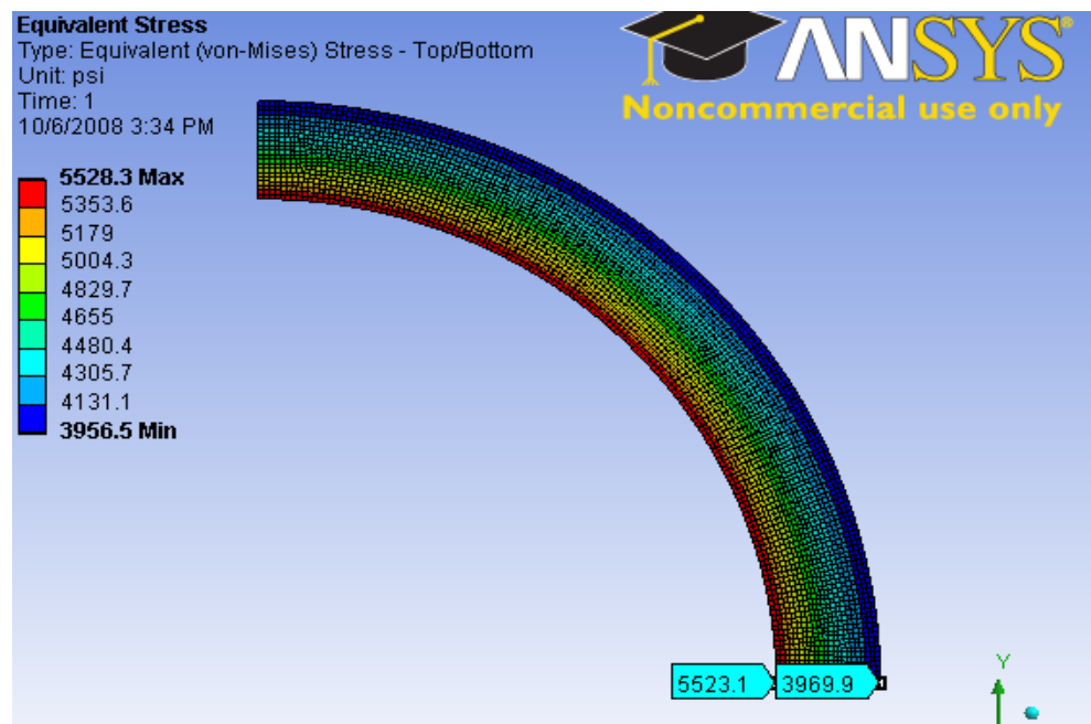
Fig 4.32: Equivalent Stress for Cement System 2 under Static loading
