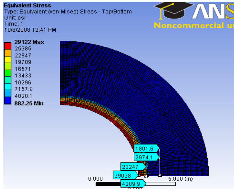
Fig 4.28: Equivalent Stress for Static Loading with Formation Property: E=1 \times 10^6 , \nu=0.3
