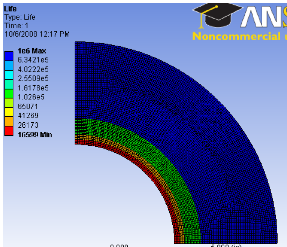
Fig 4.31: Life Cycle for Fully Reversed Loading with Formation Property: E=3 \times 10^6 , \nu=0.3
