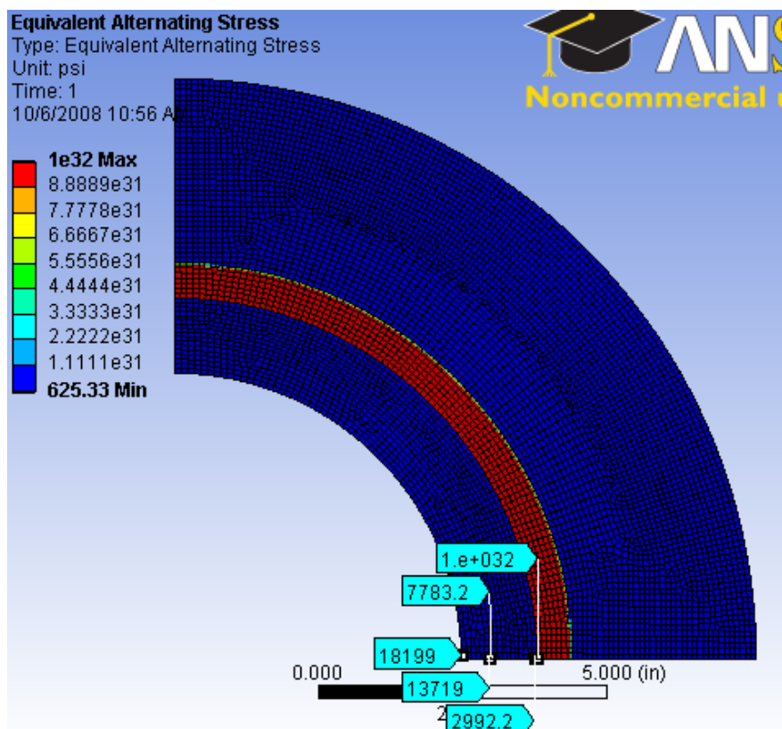
Fig 4.23: Equivalent Alternating Stress for Zero Based Loading
