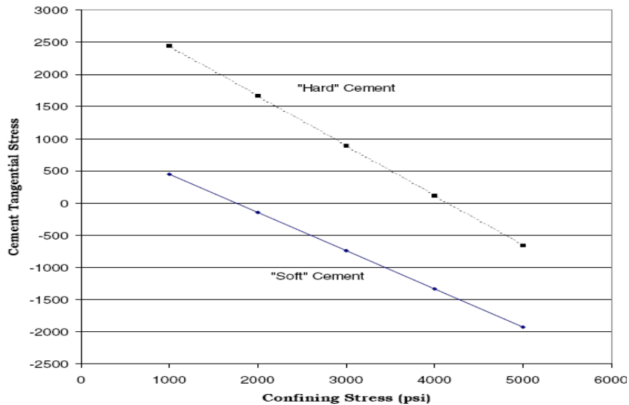
Fig 2.3: Tangential Stress for Hard and Soft Cement Systems [17]
