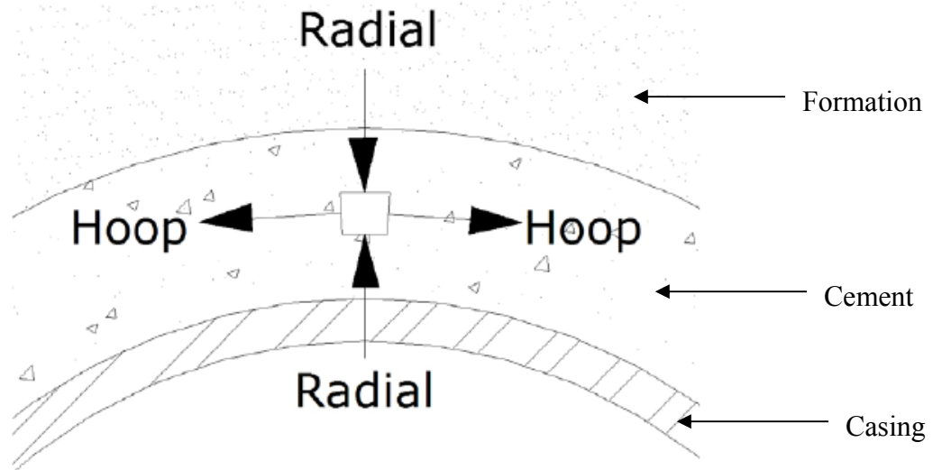
Fig 3.2: Stresses Acting on a Cement Sheath [11]
