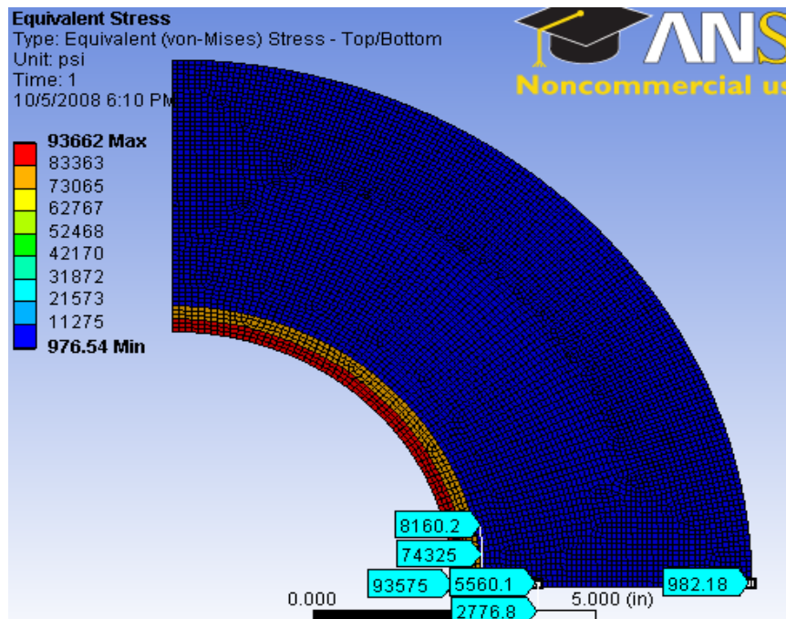
Fig 4.2: Equivalent Stress with Formation E=1 \times 10^6 psi and \nu=0.3 for Scenario 1
