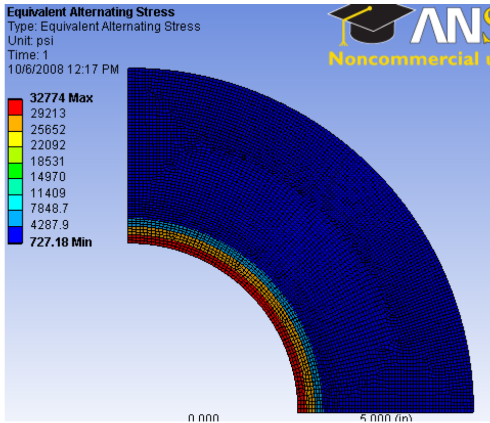
Fig 4.30: Alternating Stress for Fully Reversed Loading with Formation Property:
