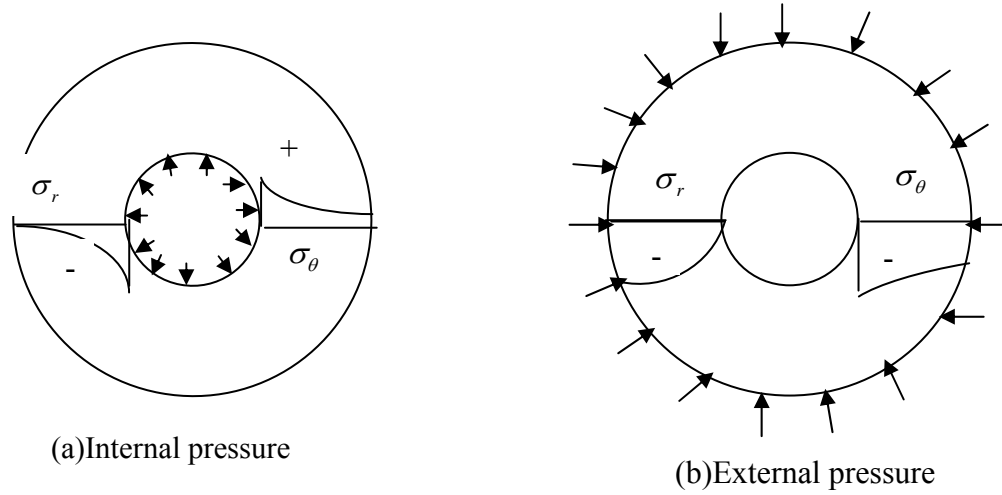
Fig 3.1: Radial and Hoop Stress Profile Due to Loading Conditions [1]
