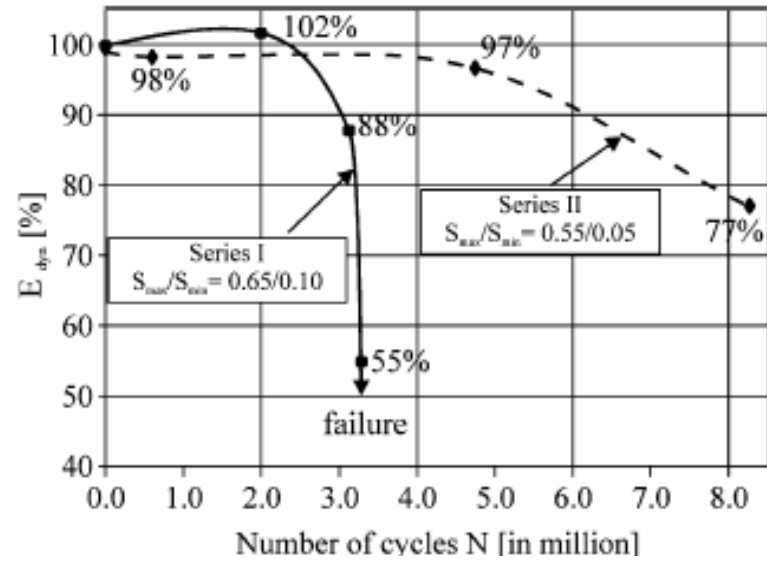
Fig 1.4: Damage Development Depending on Different Cyclic Load Levels [5]
