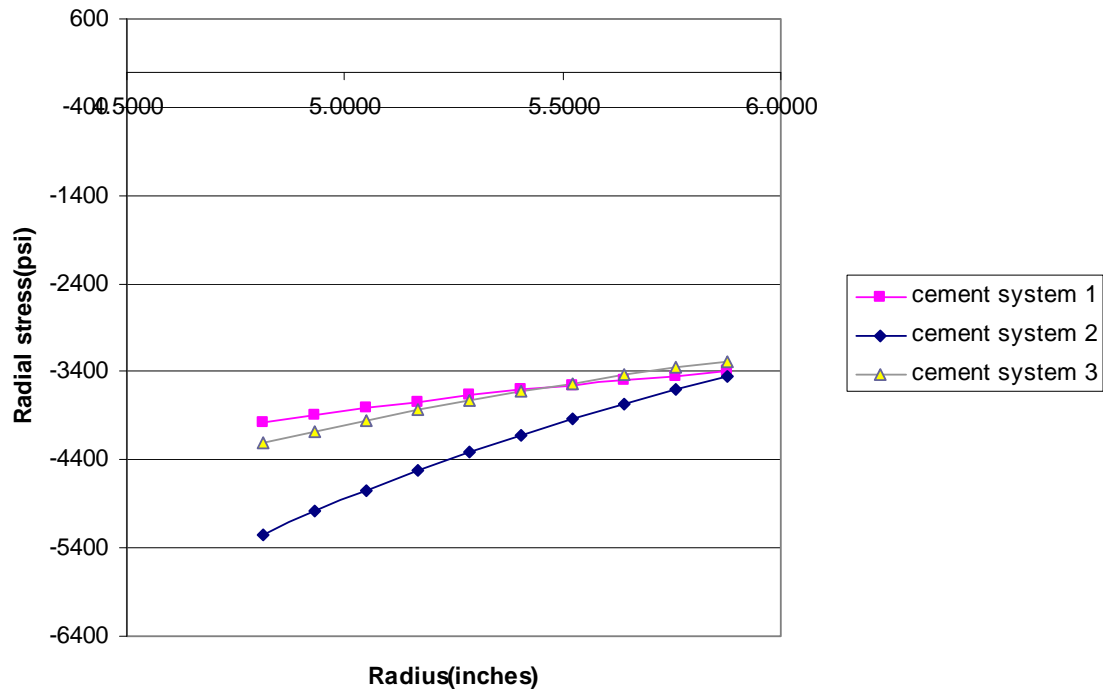
Fig 4.15: Radial Stress with p_i=15000 psi, p_f=1000 psi and \Delta T =150^\circ\text{F}
