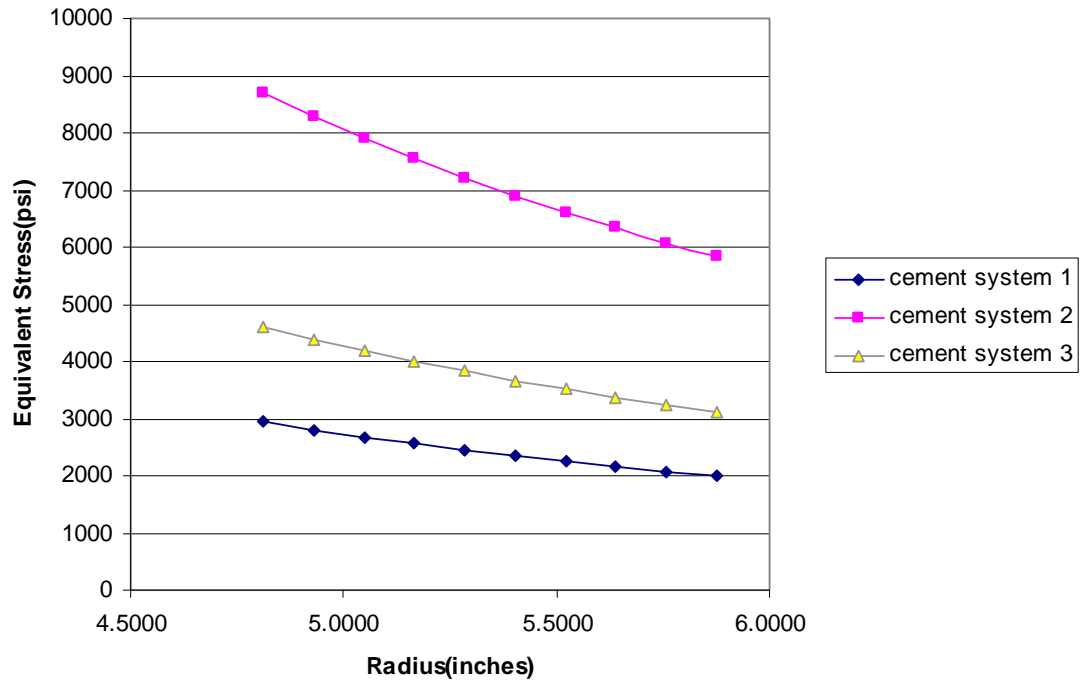
Fig 4.7: Equivalent Stress in Three Cement Systems with p_i=15000 psi and p_f=0 psi
