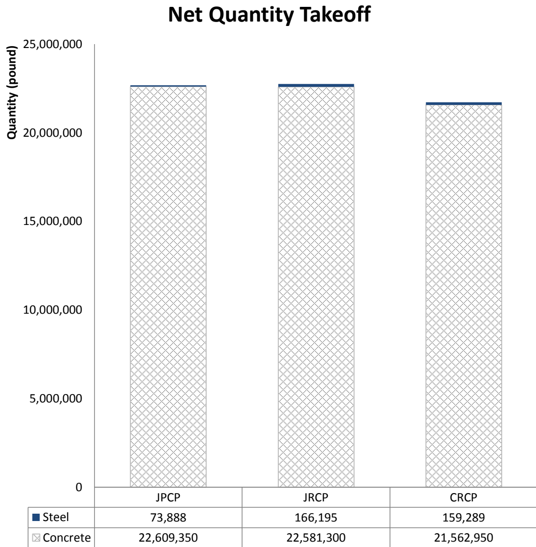
Figure 8. Concrete and Steel Quantity for JPCP, JRCP, and CRCP
