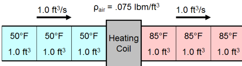
Figure 4-8 – Heating Coil Density Changes Using Packets
