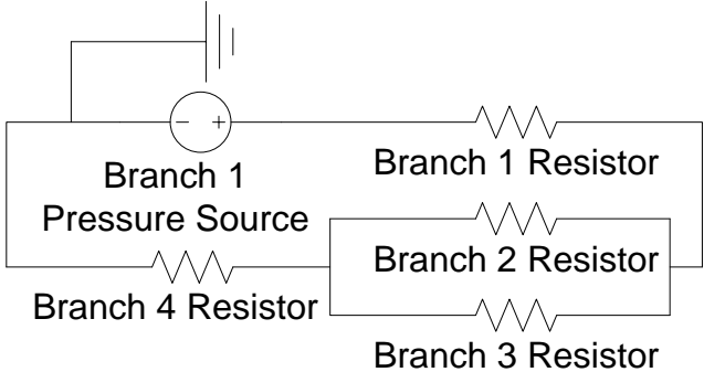
Figure 4-37 – A Branch Circuit of a Cold Water Loop
