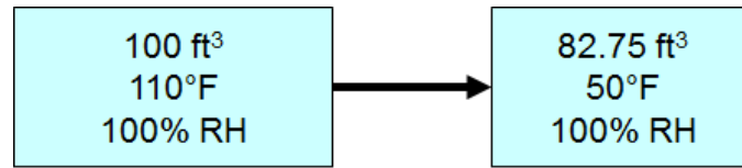
Figure 4-5 – Worst Case Cooling Density Change of Air
