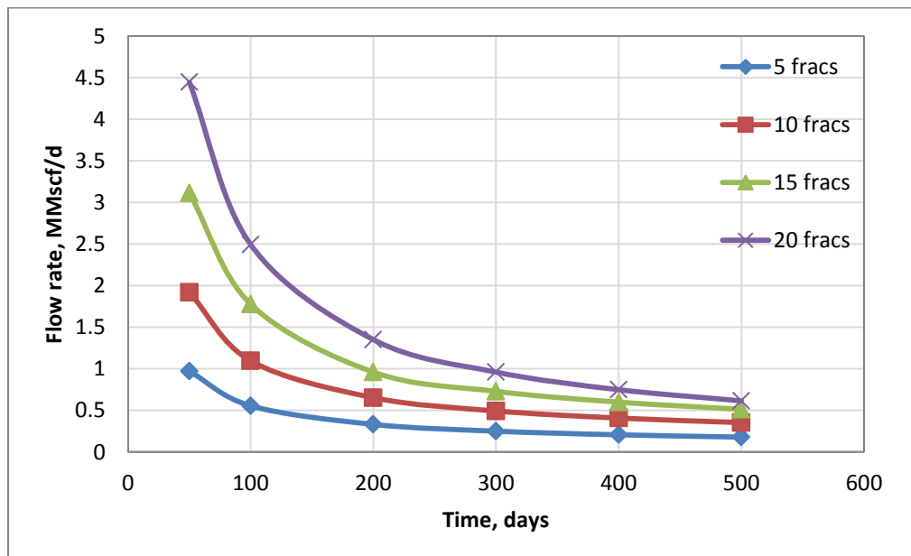
Fig. 31— Cases comparison for k_h=0.001\text{md} and k_v=0.0001\text{md} .
