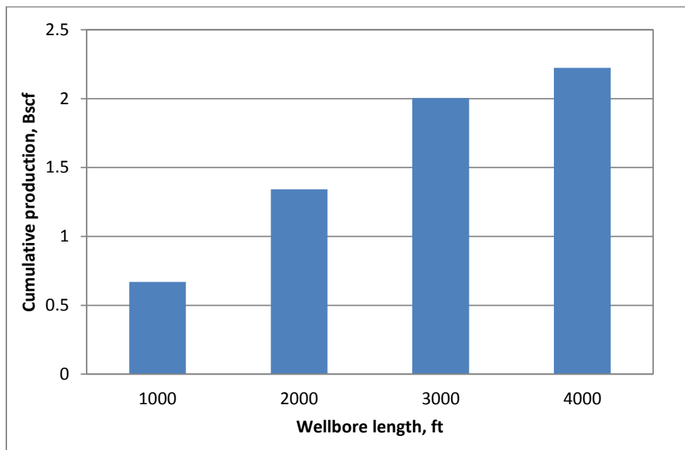
Fig. 27—Effects of wellbore length on cumulative production ( k_h=0.1\text{md} ).
