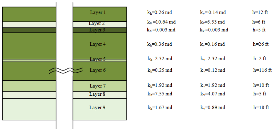
Fig. 44—Schematic of the formation.
