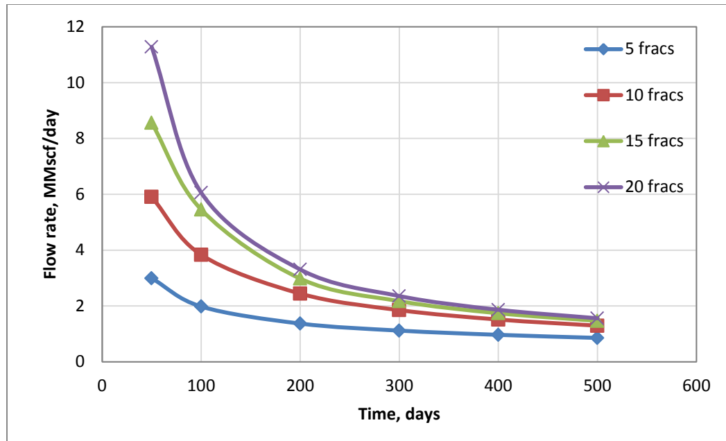
Fig. 30— Cases comparison for k_h=0.01\text{md} and k_v=0.001\text{md} .
