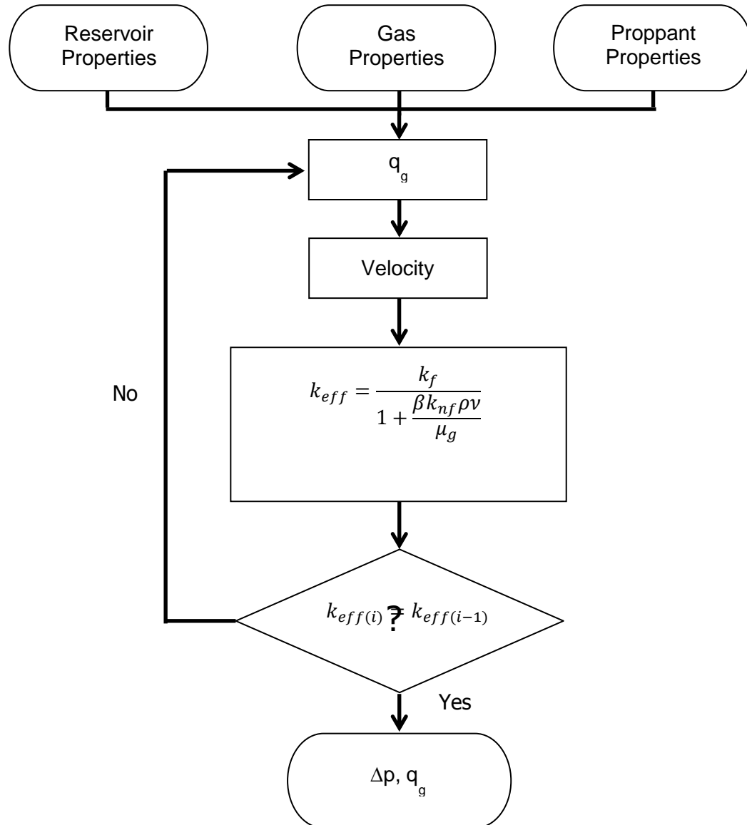
Fig. 14—Flow chart for Non-Darcy flow.
