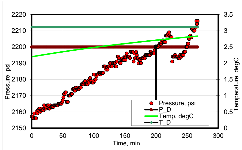
Fig. 4.2 —Estimation of drilling time to the moment, when decomposition occurs
