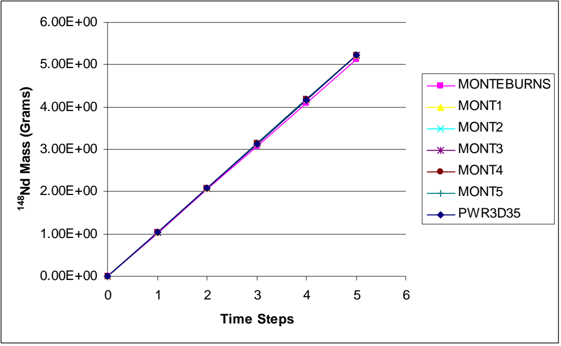
Fig. 29. Comparison of MonteBurns generated ORIGEN2 cross sections sets for 148 Nd
