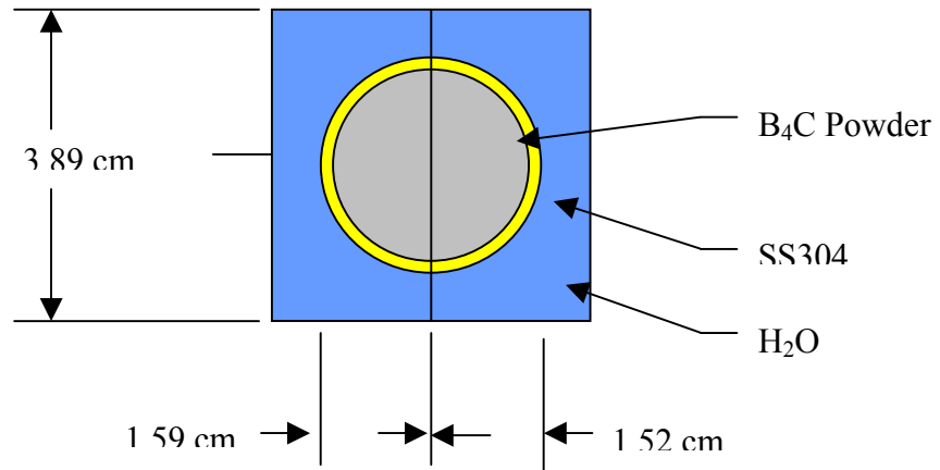
Fig. 13. Radial cross section of NSCR Regulating rod
