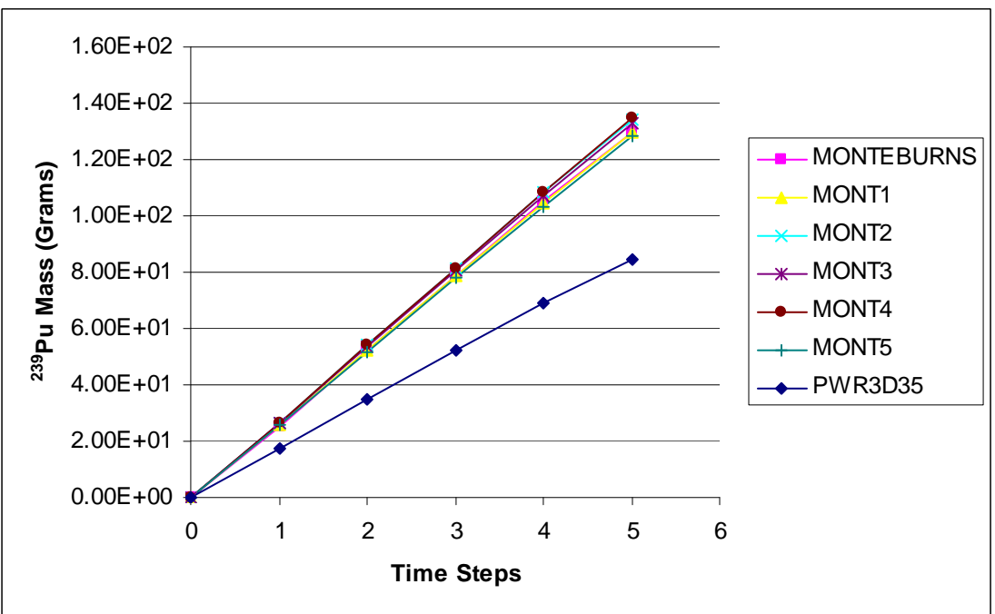
Fig. 22. Comparison of MonteBurns generated ORIGEN2 cross sections sets for 239 Pu
