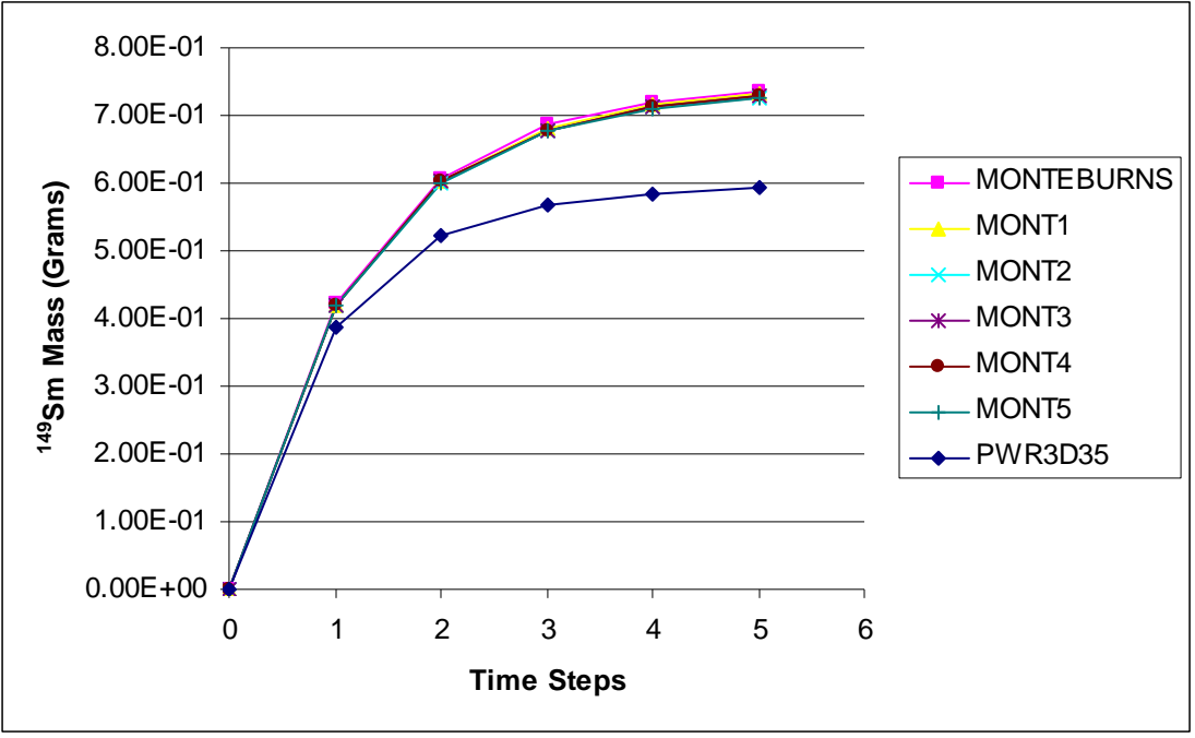
Fig. 27. Comparison of Monteburns generated ORIGEN2 cross sections sets for 149 Sm
