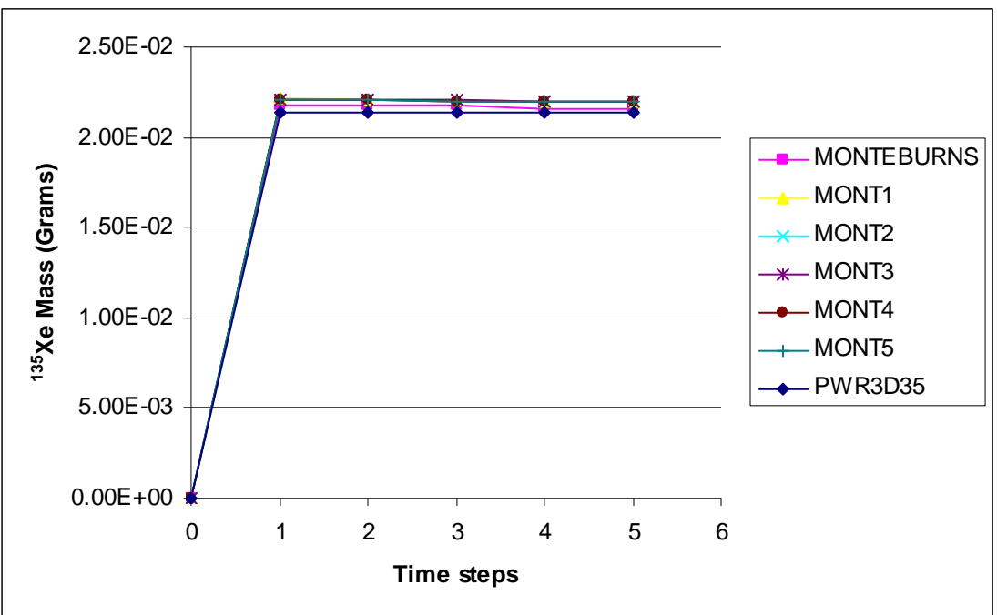
Fig. 26. Comparison of MonteBurns generated ORIGEN2 cross sections sets for 135 Xe
