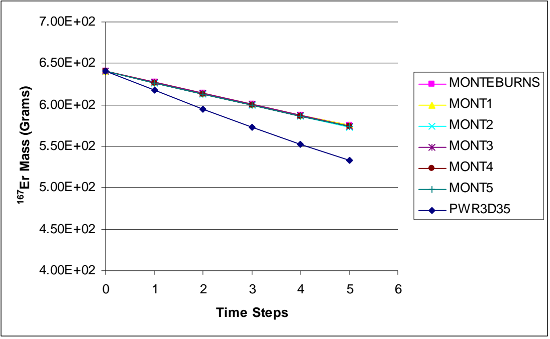
Fig. 25. Comparison of MonteBurns generated ORIGEN2 cross sections sets for 167 Er
