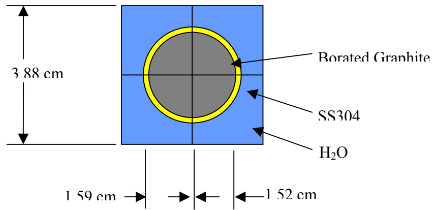
Fig. 11. Axial cross section of NSCR Transient control rod
