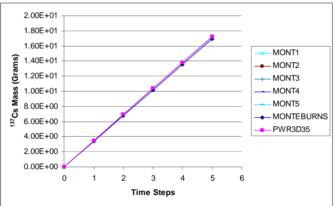
Fig. 30. Comparison of MonteBurns generated ORIGEN2 cross sections sets for 137 Cs
