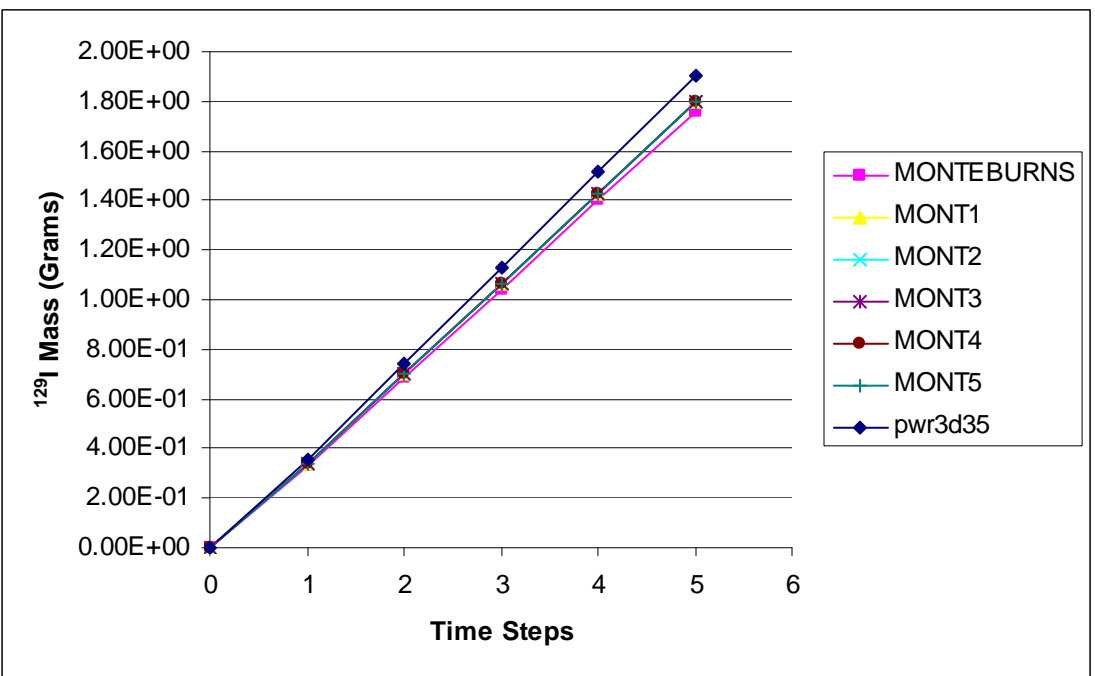
Fig. 28. Comparison of Monteburns generated ORIGEN2 cross sections sets for 129 I
