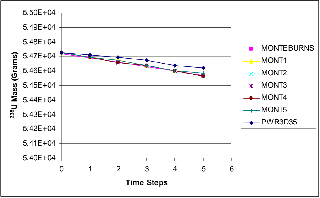
Fig. 21. Comparison of MonteBurns generated ORIGEN2 cross sections sets for 238 U
