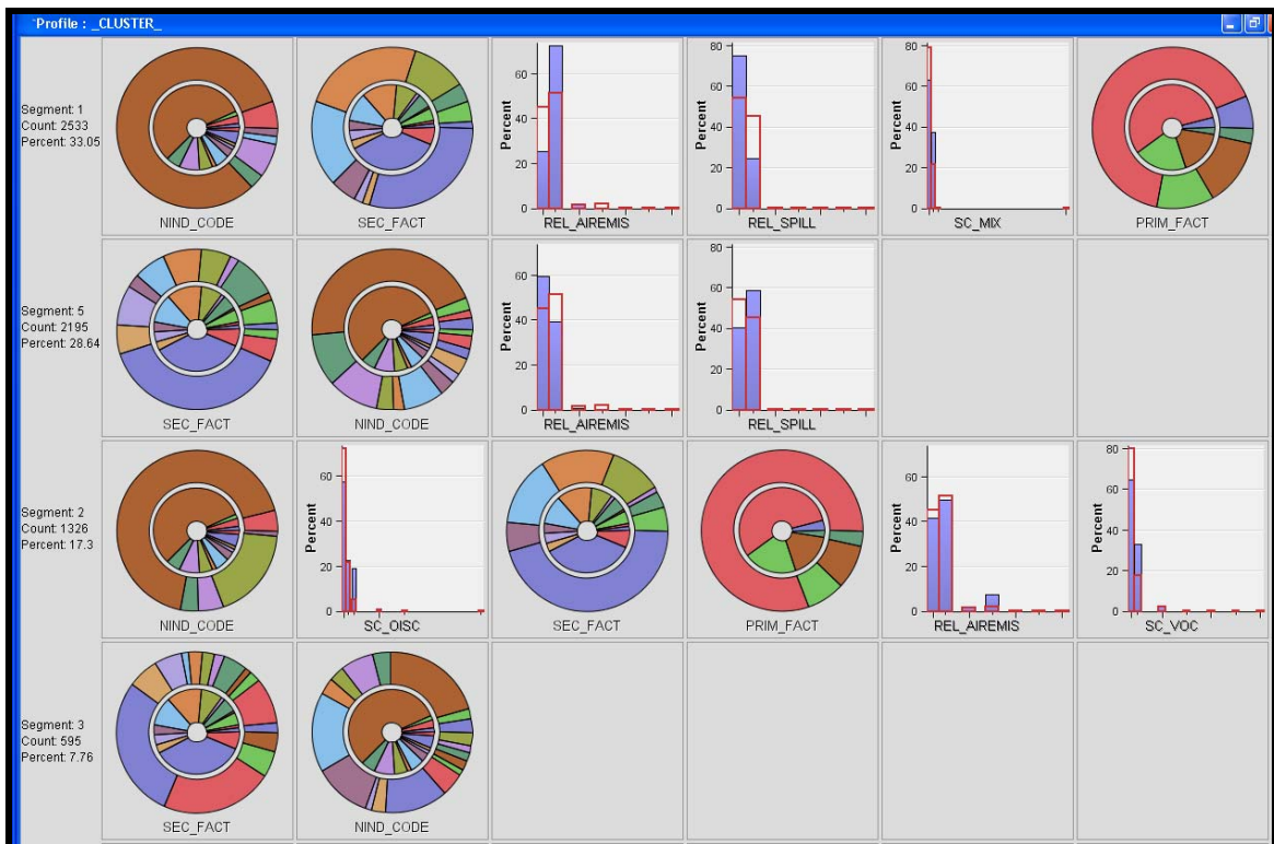
Figure 9 Cluster Rings
