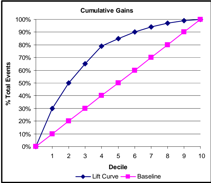
Figure 1 Example of Cumulative Gain Chart
