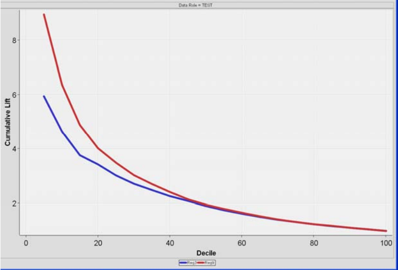
Figure 12 Cumulative Lift Comparison for Test Dataset
