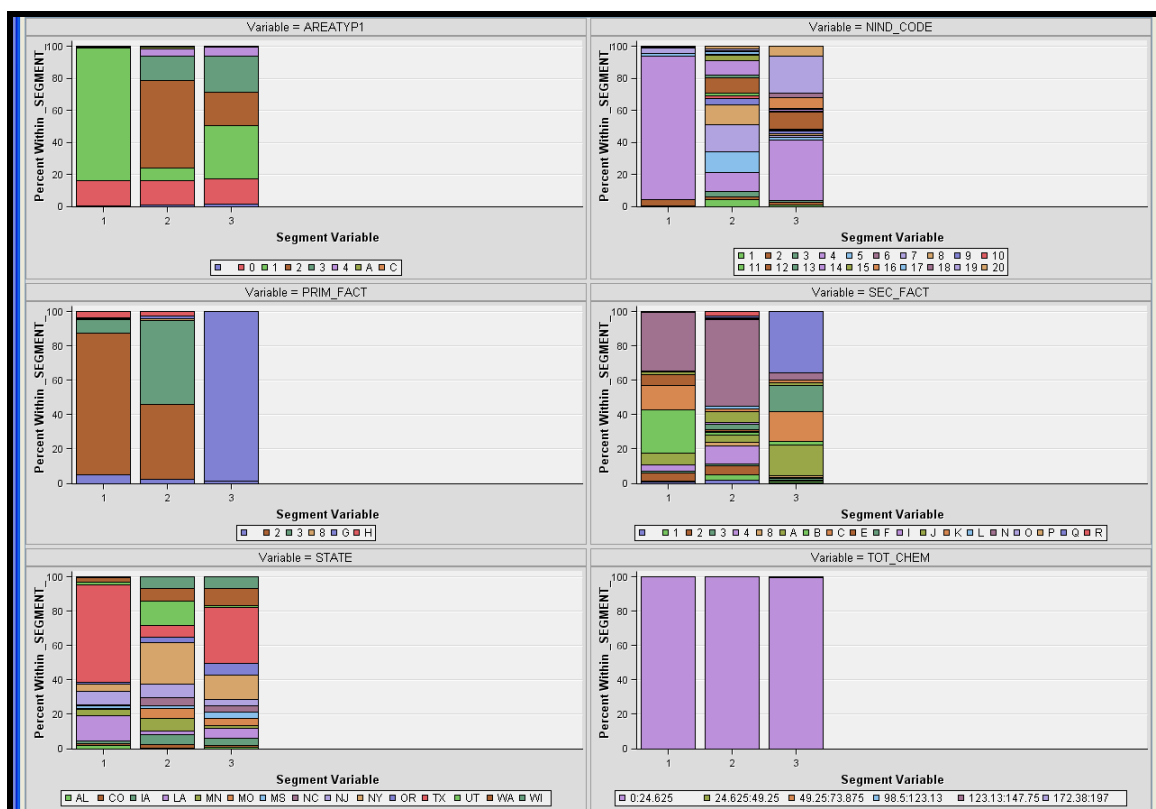
Figure 8 Clustered Data
