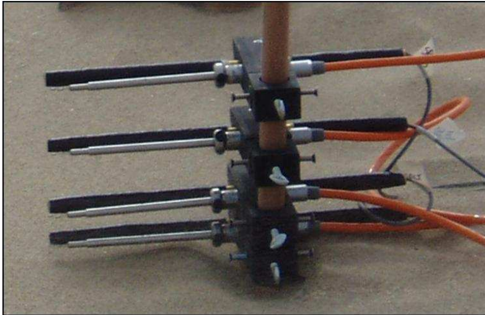
Fig. 3-10. Thermal anemometers (silver) and miniphones (black) mounted on an instrument tower at 0.02, 0.06, 0.12, and 0.20 m above the bed. A portion of a sand trap can be seen on the top of the photograph. This photograph was taken during a Configuration A run. Only the bottom TA-MIC pairs are used in this research.
