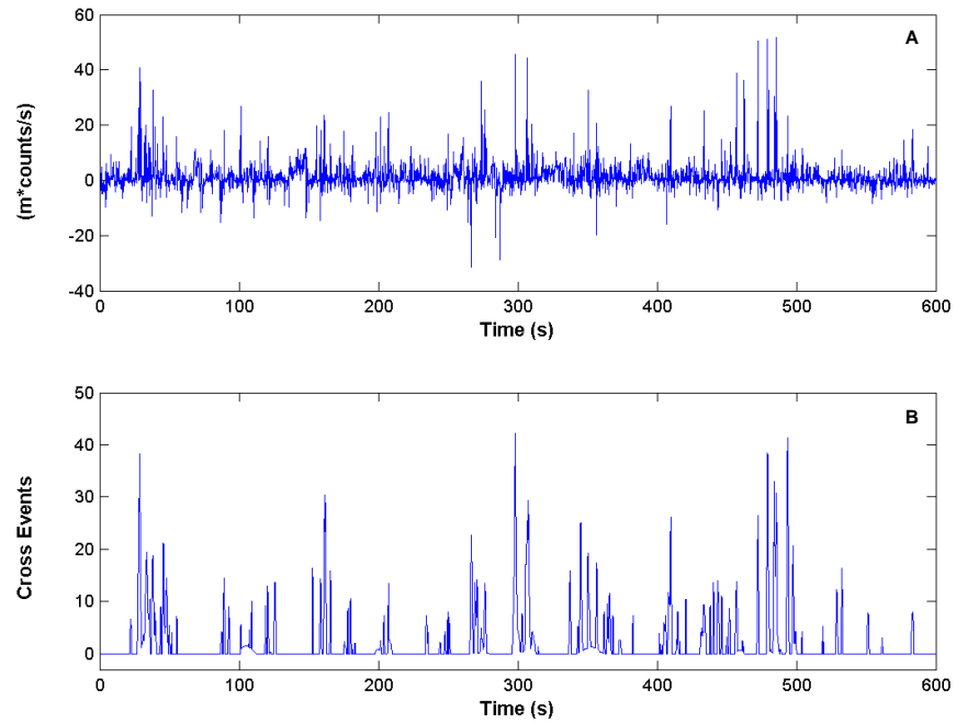
Fig. 5-32. The complex conjugate of the wind and sand 5 Hz demeaned time series from Run 4 (A) and the corresponding cross wavelet events (B).
