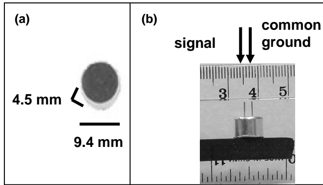
Fig. A-2: The miniphone as produced by the manufacturer. Unit diameter is 9.4 mm and depth is 4.5 mm (a). Backside of instrument has pins to connect leads (wires) for the miniphone output signal and common ground (b).
