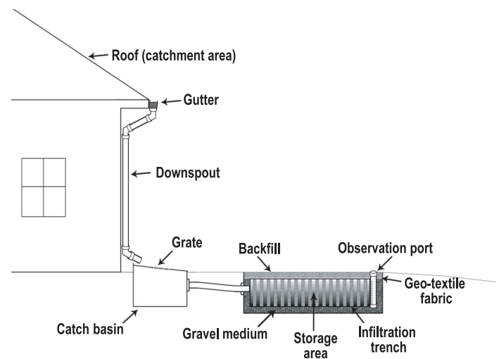
Figure 1. Rainwater soil storage and infiltration system components.
