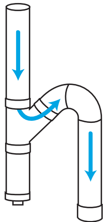
Figure 4. Diagram of a “poor man’s” roof washer.
