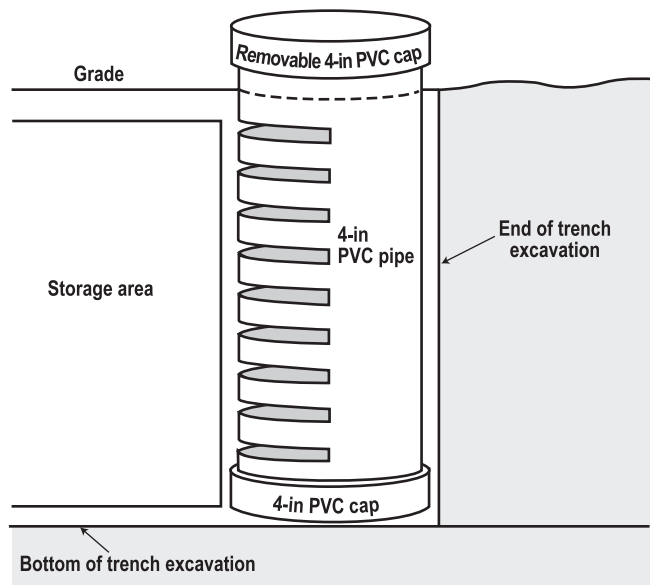
Figure 8. Placement of an observation port in a soil storage and infiltration system (drawing not to scale).
