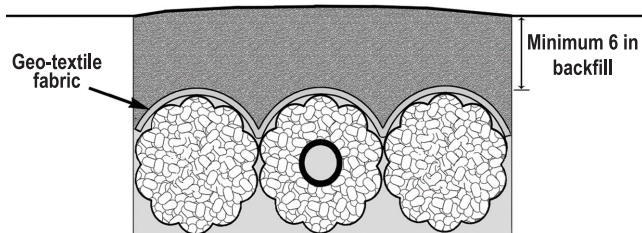
Figure 7. Trench construction using polystyrene media.
