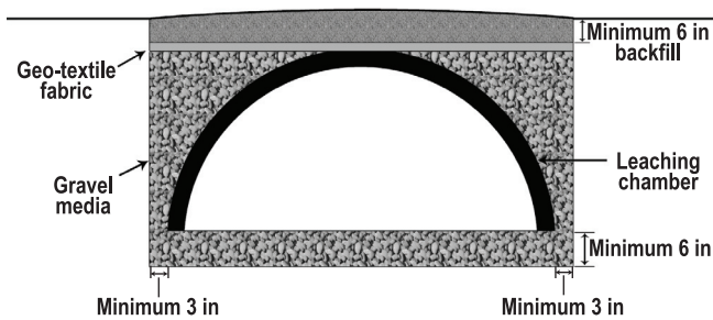
Figure 6. Trench construction using a leaching chamber.
