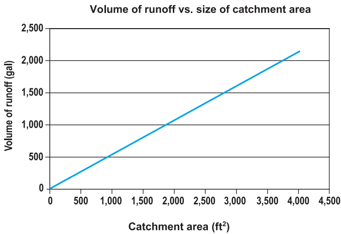
Figure 3. Relationship between catchment size (ft 2 ) and runoff volume (gal) (assuming 85 percent of the runoff is collected from a 1-inch rain).
