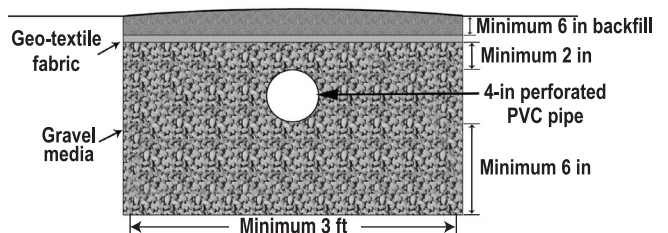
Figure 5. Trench construction using a gravel media with perforated pipe.
