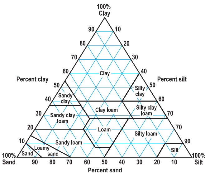
Figure 2. Soil texture triangle (USDA, 1993).
