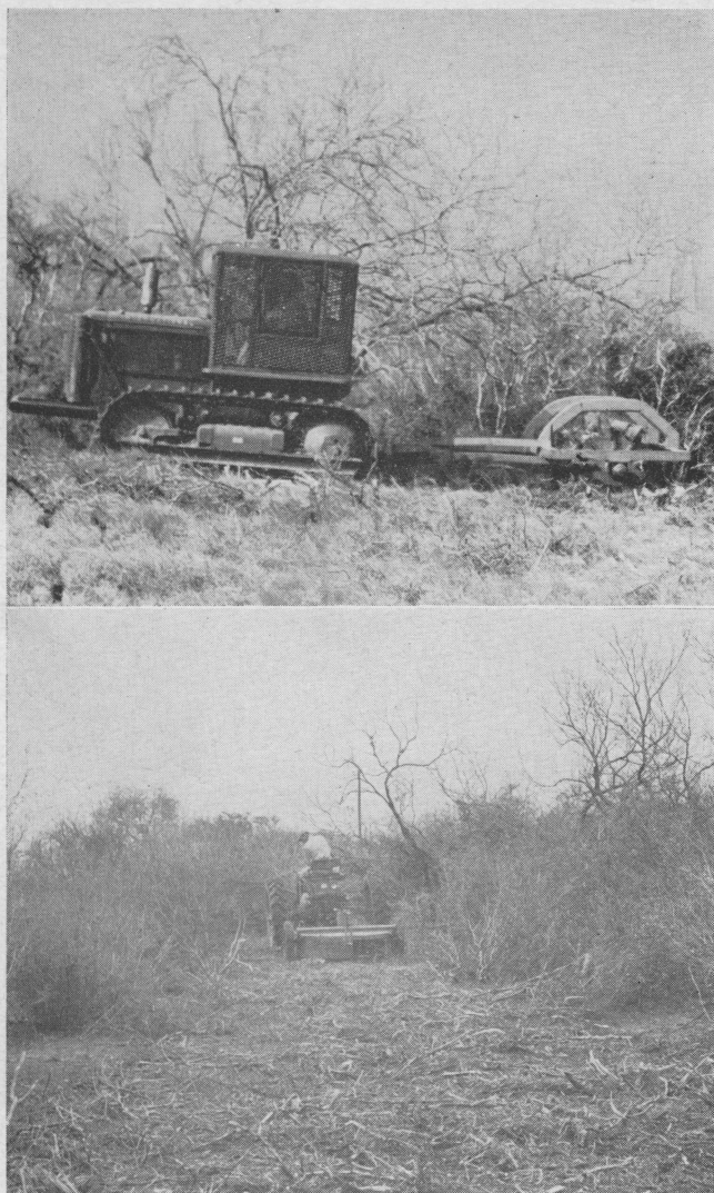
Figure 12. Above—Heavy-duty brush cutter weighing 14,000 pounds used to crush and chop mixed brush. Below—Rotary shredder used to cut underbrush. Chemicals are not effective for the control of mixed brush. Courtesy E. L. Caldwell Manufacturing Co., Corpus Christi, Texas.
