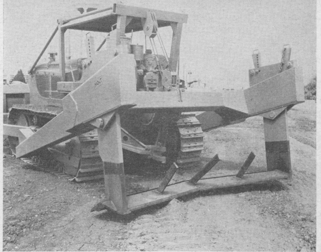
Figure 13. Above—Heavy-duty brush plow with fins on the cutting blade that help lift roots of underbrush out of the soil. Below—Giant heavy-duty brushplow used on the King Ranch. These plows are equipped with seeders that utilize the exhaust to plant grass seed at the time of plowing. Courtesy of the Holt Manufacturing Company, San Antonio, Texas, and the King Ranch, Kingsville, Texas.
