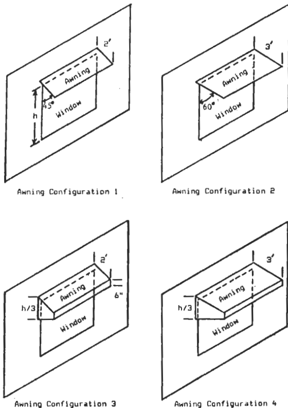
Figure 2: Awning Configurations
