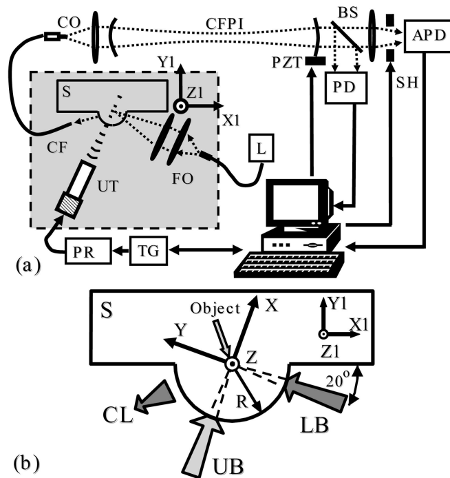
Fig. 2.1. Experimental setup. (a) Schematic of the experimental setup: L, laser; TG, trigger generator; PR, pulserreceiver; UT, ultrasonic transducer; FO, focusing optics; CF, collecting fiber; S, sample; CO, coupling optics; PZT, piezoelectric transducer; BS, beam splitter; SH, shutter; PD, photodetector. (b) Top view of the sample (S): UB, ultrasound beam; LB, incident light beam; CL, collected light; R, radius of curvature. Other abbreviations defined in text.
