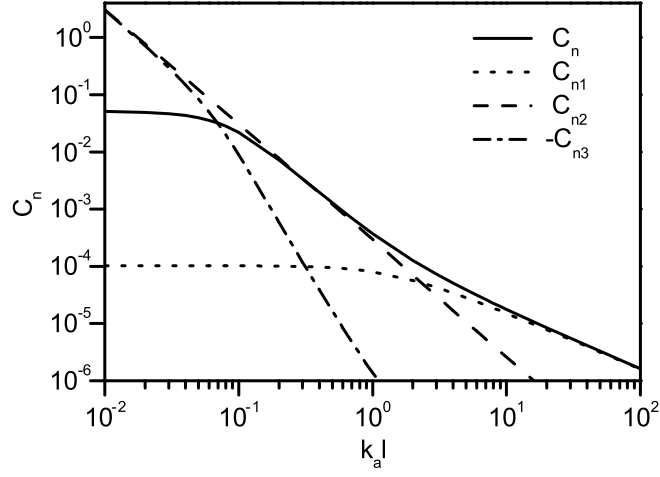
Fig. 4.2. Dependence of the components of the C_n term on the ultrasound frequency, for s/l = 10^3 . The values of the parameters used are: l = 1 mm, \Lambda = 1 m ^{-1} , \eta = 0.32 , S = 1 , and \phi = 0 .
