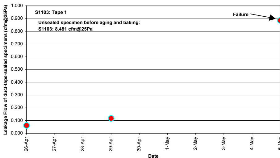
Figure 12. The Measured Leakage of the Collar-to-Plenum Joint Tape-1 Specimen
