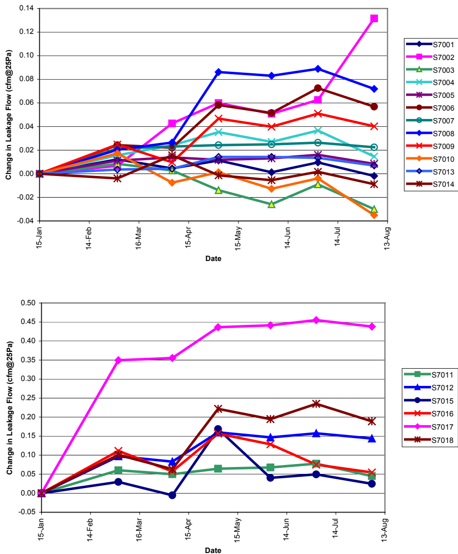
Figure 10 (a and b). The Measured Change in Leakage Flow of the Flexible Core To Sheet Metal Collar Joint Specimens During the Six-Month Period of the Aging Test
