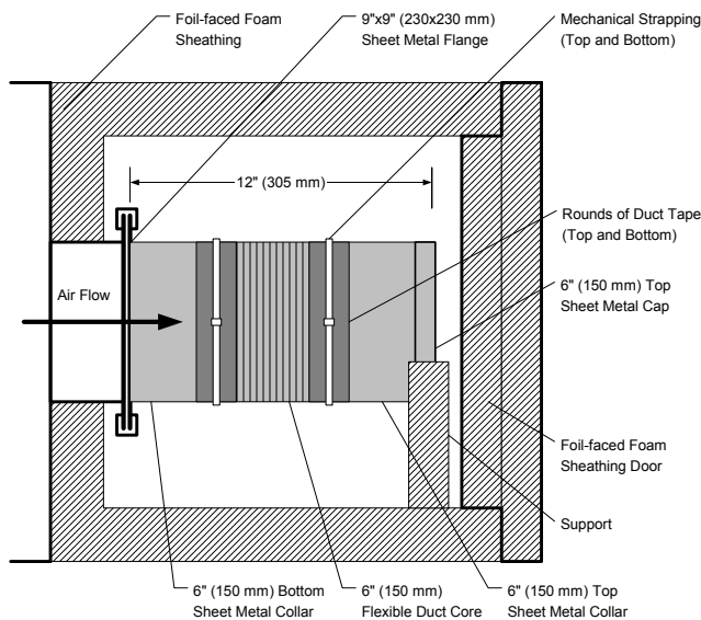
Figure 6. A Side-View Schematic of a Flexible Duct Core to Sheet Metal Collar Joint Specimen Positioned on the Aging Test Apparatus
