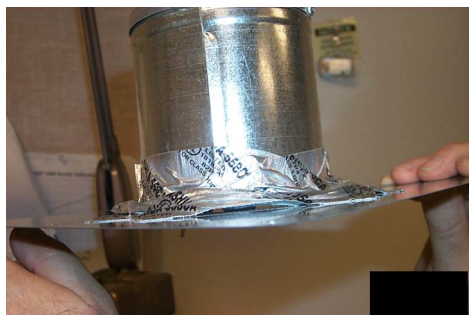
Figure 13. A Typical Failure of the 3-D Collar-To-Plenum Joint
