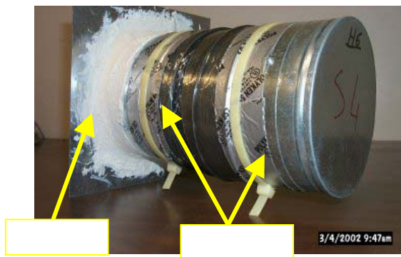
Figure 5. Example of Test Sample Showing the Two Taped Connections and the Mechanical Clamps
