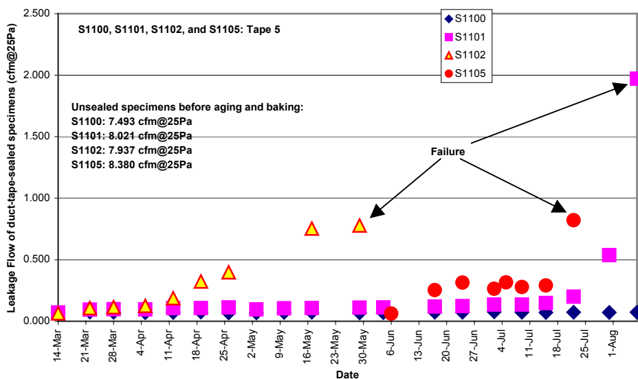
Figure 11. The Measured Leakage of the Collar-To-Plenum Joint Tape-5 Specimens
