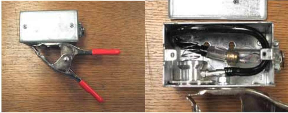
Figure 5. Acoustic sensor (Seo, 2003)
