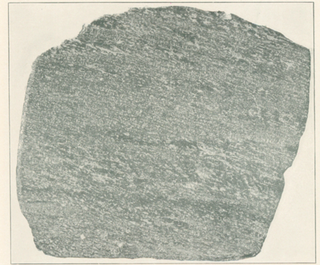
PLATE XII.—POLISHED SURFACE OF PINK AND BLUE RHYOLITE.
