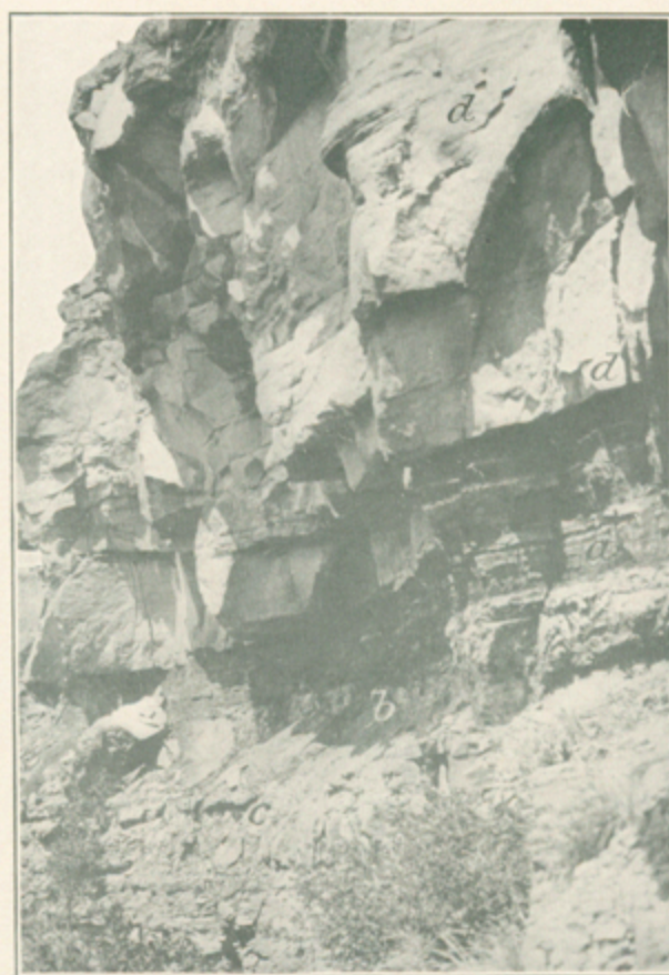
PLATE X.—RELATION OF THE WILLOW COAL BED TO OTHER BEDS WHERE THE VERMEJO FORMATION IS THIN. The coal bed (a), here about 5 feet thick, is separated by a few feet of shale (b) from the underlying Trinidad sandstone (c). The basal conglomerate (d) of the Raton formation rests with uneven base directly on the coal.
