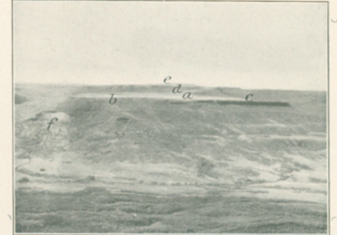
PLATE VI.—HORSESHOE AND BARILLA MESAS AS SEEN FROM JOHNSON MESA. a, Smooth surface of Horseshoe Mesa; b, c, edge of the sheet of basalt (thin at b, thick at c) which caps the mesa; d, narrow neck connecting Horseshoe Mesa with the higher Barilla Mesa; e, volcanic cone on Barilla Mesa from which the lava capping Horseshoe Mesa was probably extruded; f, recent landslide on steep slope of mesa.
