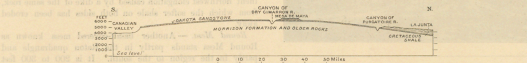
FIGURE 6.—Section across the Mesa de Maya dome from Canadian Valley on the south to La Junta, Colo., on the north. Shows the doming of the Cretaceous rocks. Mesa de Maya is capped by Tertiary lava.
