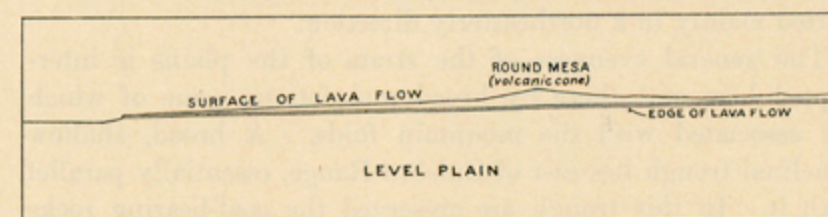
FIGURE 9.—Lava-capped Round Mesa and associated volcanic cone.
