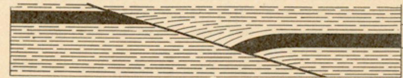
FIGURE 16.—Sketch of normal fault in Willow mine, south of Van Houten. The coal bed, which has been dropped about 15 feet, is bent downward on the downthrown side of the fault, as if it had been subjected to compression and slight upthrusting after the original faulting.
