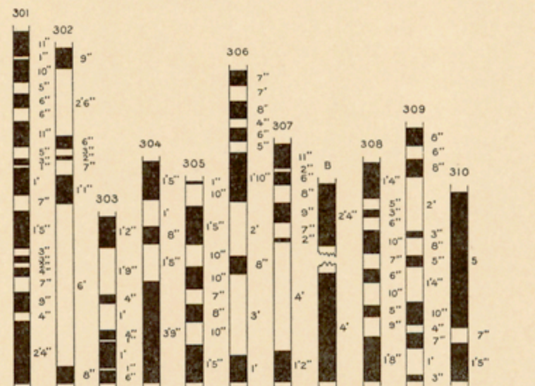
FIGURE 21.—Sections of coal beds in the Raton and Vermejo formations in the southwestern part of the Brilliant quadrangle. Black bands represent coal. Numbers above columns indicate localities marked on economic-geology map where sections were measured.
