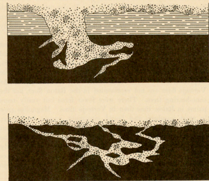
FIGURE 15.—Sketches showing the relation of the basal conglomerate of the Raton formation to the underlying shale and coal of the Vermejo formation in the mine face of the Willow mine, near Van Houten. The conglomerate seems to fill irregular crevices in the upper surface of the coal and associated shale of the Vermejo formation.
