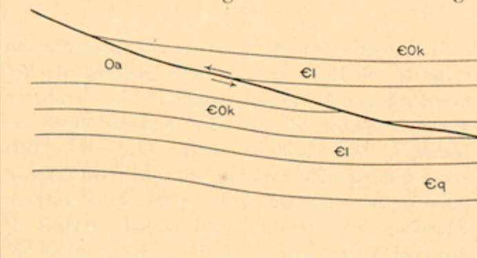
FIG. 3.—Theoretical section showing supposed relations of beds in fig. 2 after the major faulting but before the later folding and faulting.
