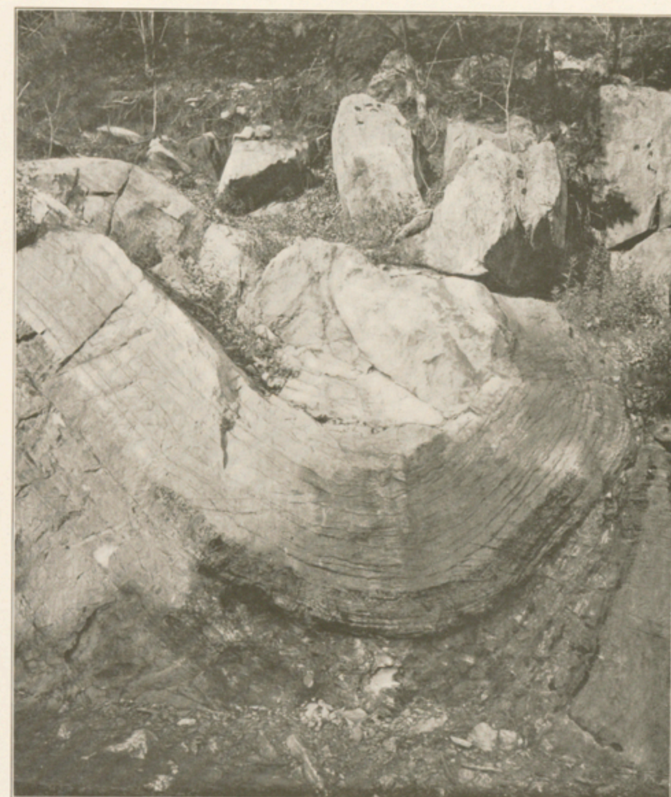
FIG. 9.—CLOSE FOLDING IN MASSIVE BLUE KNOX DOLOMITE ALONG NOLICHUCKY RIVER NORTHEAST OF EMBREEVILLE, TENN.
