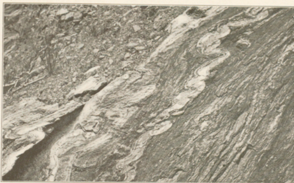
FIG. 7.—GRANITOID GNEISS WITH FOLDED QUARTZOSE LAYERS, 5 MILES EAST OF BIG YELLOW MOUNTAIN.
