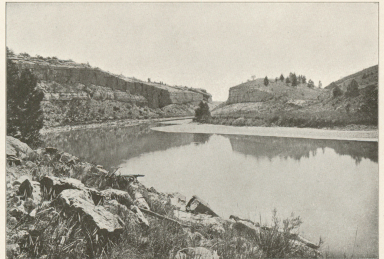
FIG. 4.—CANYON OF NORTH PLATTE RIVER WEST OF FAIRBANK, LOOKING EASTWARD. Showing the massive quartzite at the base of the Hartville formation resting unconformably on the bedded rocks of the Guernsey formation.
