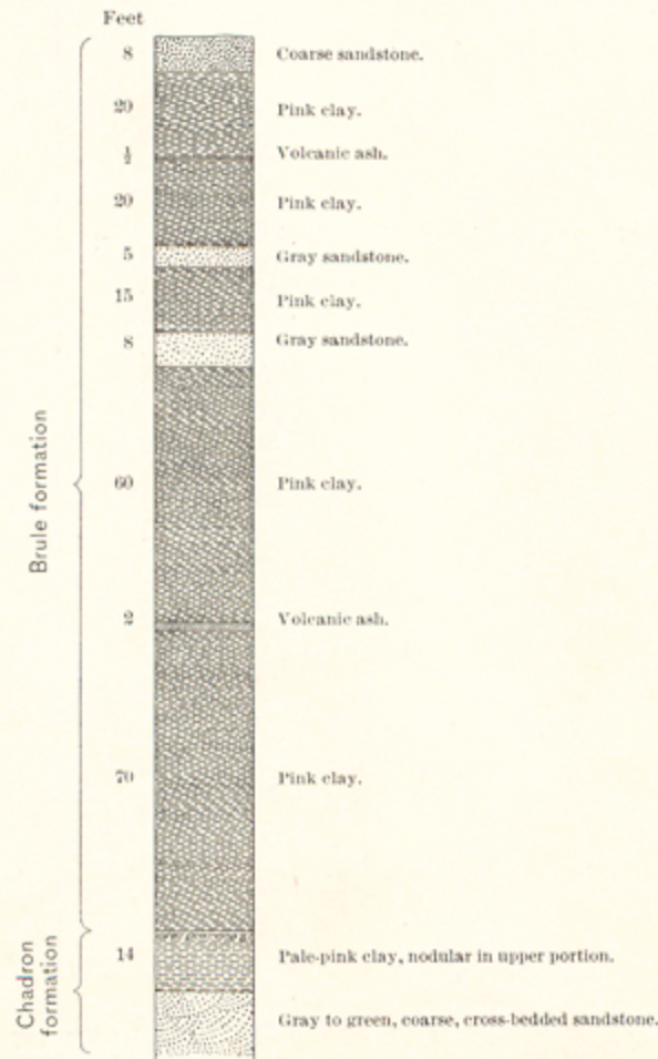
SECTION 2. BRULE FORMATION, 1 1/2 MILES SOUTH- WEST OF DOTY'S RANCH.
