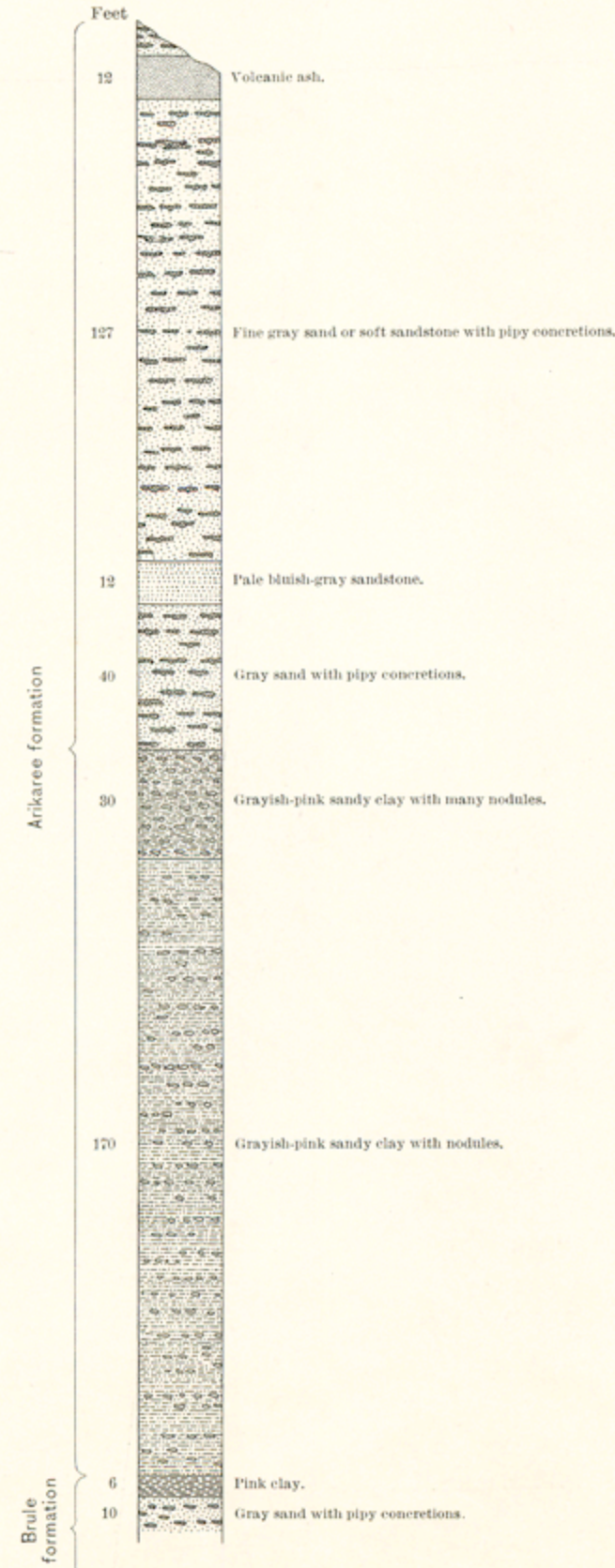
SECTION 3. BASAL PORTION OF ARIKAREE FORMATION, 1 MILE SOUTH- WEST OF LAKEVIEW.
