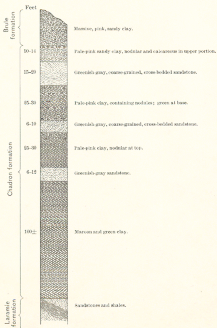
SECTION 1. CHADRON FORMATION, WESTERN PORTION OF GOSHEN HOLE.
