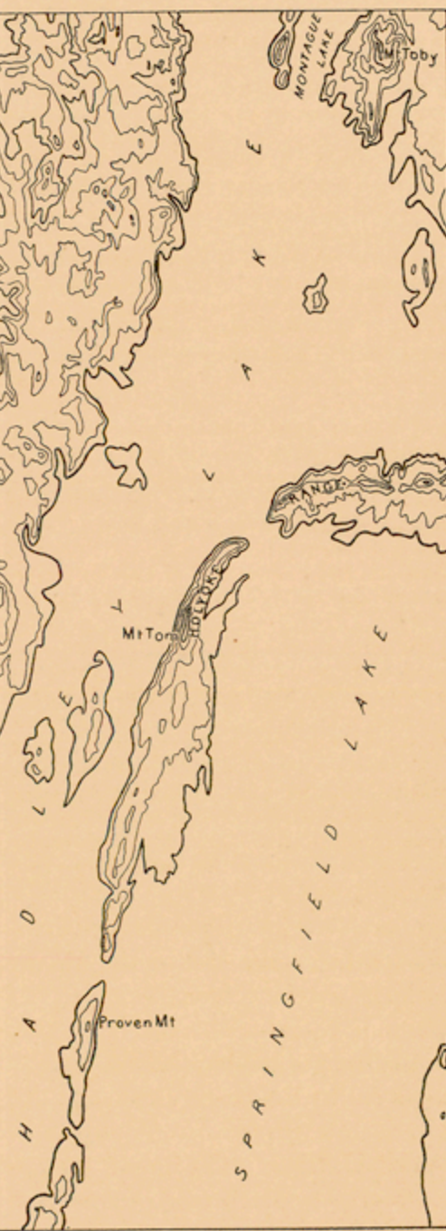
FIG. 2.—THE CONFLUENT GLACIAL LAKES OF THE CONNECTICUT VALLEY. A MAP OF THE HOLYOKE QUADRANGLE, SHOWING THE POSITION OF THE THREE GLACIAL LAKES WHICH OCCUPIED THE CONNECTICUT VALLEY DURING THE RETREAT OF THE ICE. THE TOPOGRAPHY OF THE LAND AREAS IS THAT OF THE PRESENT SURFACE, REPRESENTED IN CONTOURS OF 200-FOOT INTERVAL, REFERRED TO THE PRESENT SEA LEVEL AS A DATUM PLANE.
