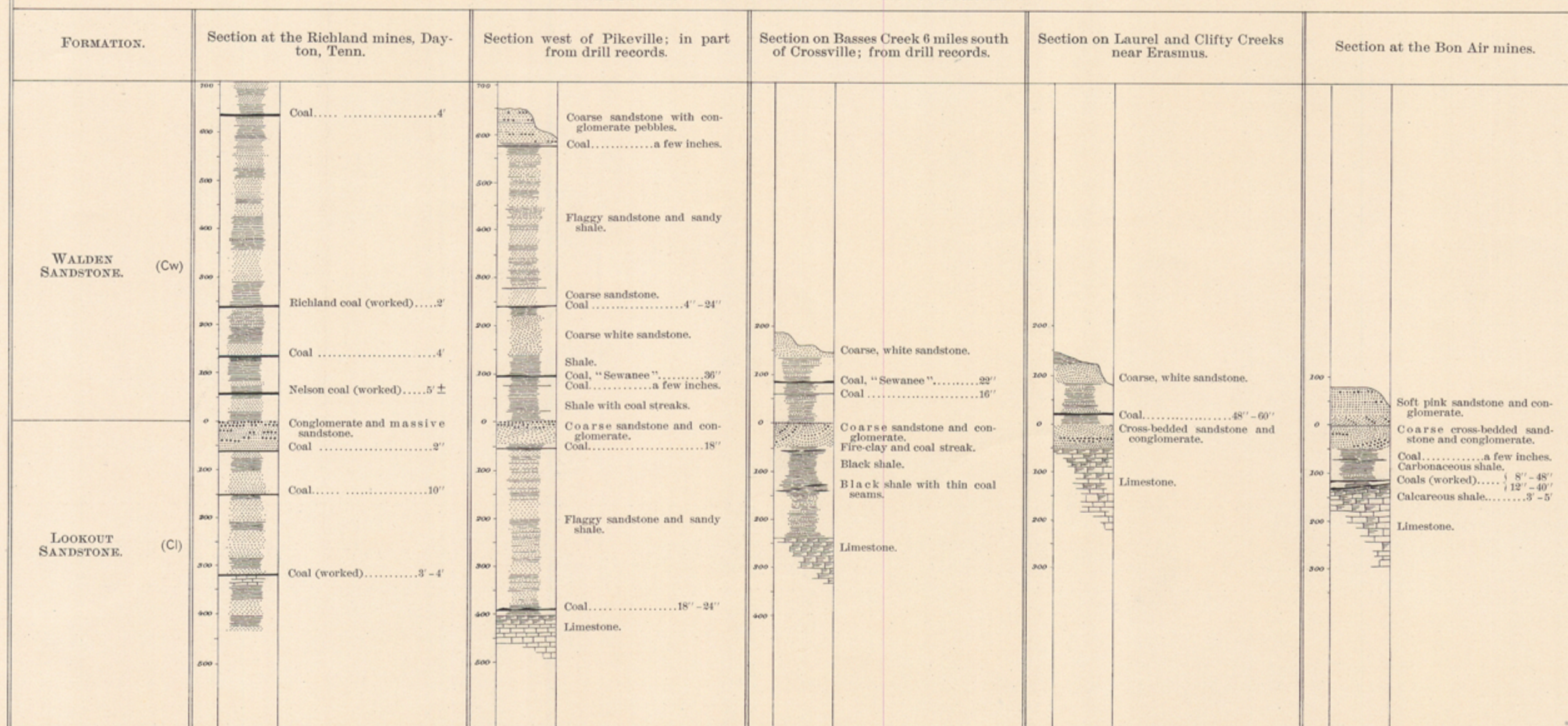
VERTICAL SECTIONS; SHOWING THE POSITION AND THICKNESS OF COAL BEDS. SCALE: 250 FEET = 1 INCH. VERTICAL DISTANCES ARE MEASURED FROM THE TOP OF LOOKOUT CONGLOMERATE.
