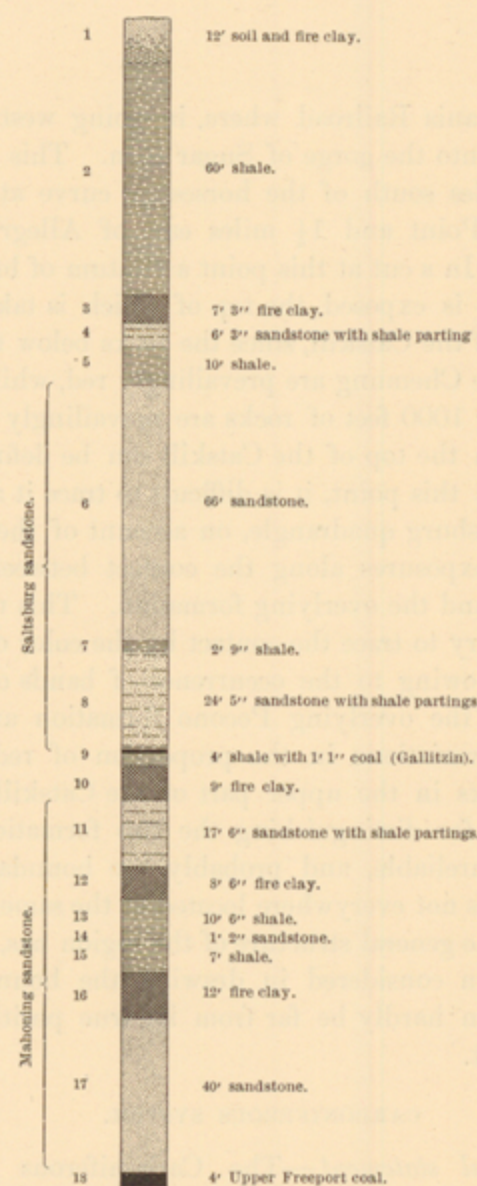
FIG. 6.—Section of Cresson mine shaft, Cresson, Pa.
