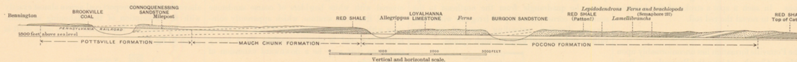
FIG. 3.—Profile section of Mississippian and Pottsville rocks along Pennsylvania Railroad on the Allegheny Front west of Altoona.
