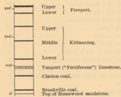
FIG. 3.—Section showing coal beds of the Allegheny formation in the Allegheny Valley.
