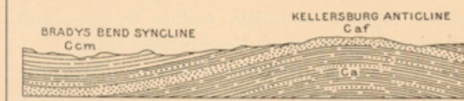
FIG. 2.—Ideal section illustrating planation of folded rocks. Vertical scale and dips greatly exaggerated.
