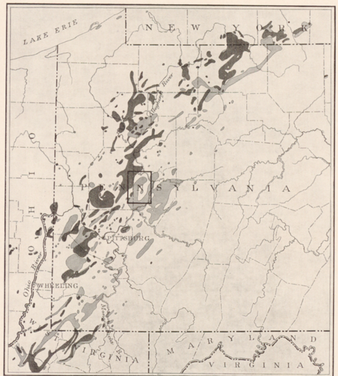
FIG. 12.—MAP OF THE OIL AND GAS PRODUCING AREAS OF THE NORTHERN APPALACHIANS. Compiled from map by the Second Geological Survey of Pennsylvania, and from maps by the United States Geological Survey. Dark areas, oil; lighter areas, gas. The location of the Kittanning quadrangle is shown by the rectangle.
