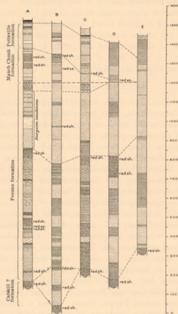
FIG. 5.—Columnar sections of the Mississippian and Pottsville rocks in western Pennsylvania.
