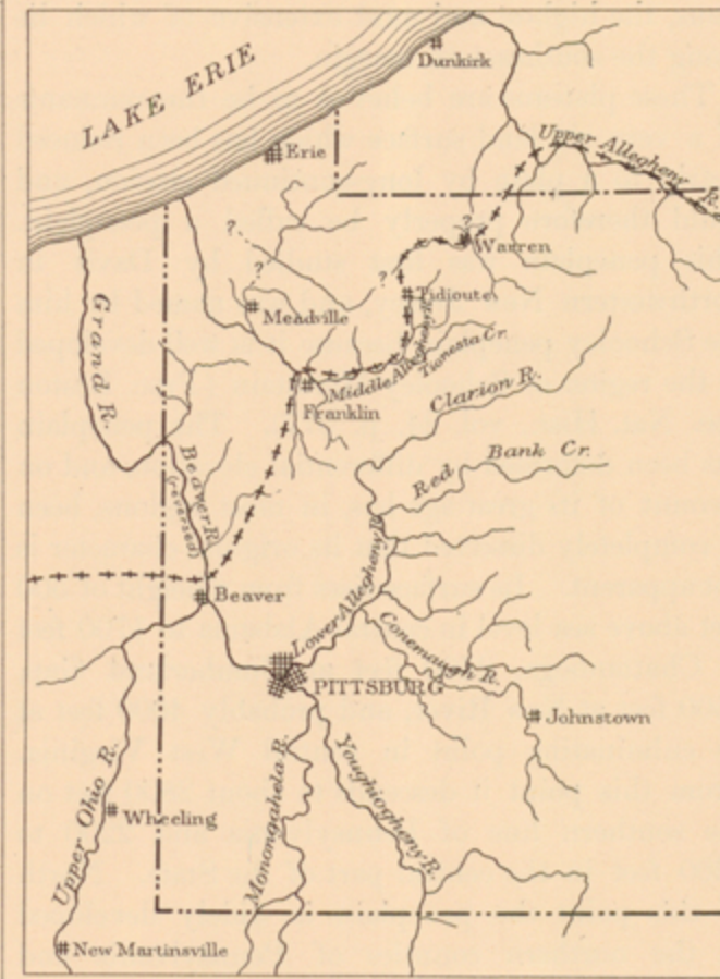
FIG. 1.—Sketch map showing the probable pre-glacial drainage of western Pennsylvania. The terminal moraine is shown by a broken crossed line. (After Frank Leverett; with addition of terminal moraine.)
