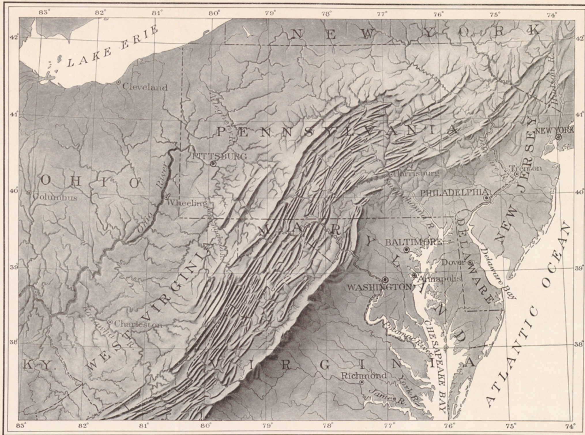
FIG. 10.—RELIEF MAP OF THE NORTHERN APPALACHIAN MOUNTAINS. The Kittanning quadrangle is situated on the plateau lying west of the belt of valley ridges, in the west-central part of Pennsylvania.
