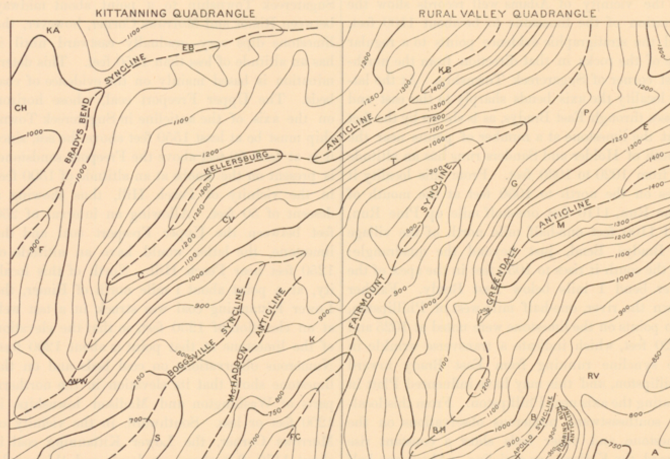
FIG. 4.—Map of Kittanning and Rural Valley quadrangles showing the geologic structure by means of contour lines drawn on the top of the Vanport ("Ferriferous") limestone. Contour interval, 50 feet.
