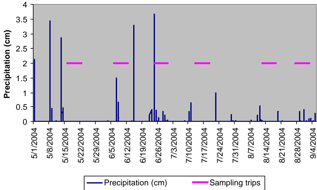
Fig. 5. Precipitation.
