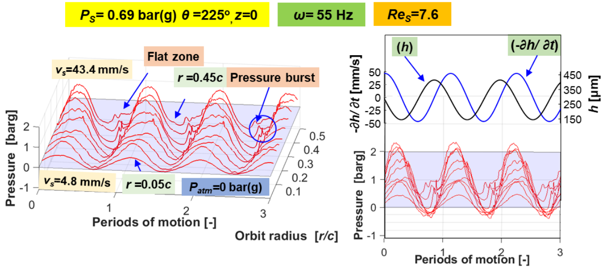
(a) Cascade plot of dynamic pressures for \omega = 55 \text{ Hz} : isometric view
