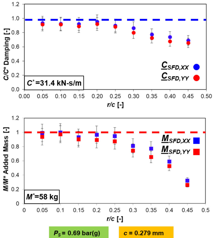
Figure 18. Experimentally identified normalized SFD force coefficients ( \underline{C}_{SFD} , \underline{M}_{SFD} ) _{XX,YY} vs. orbit radius ( r ). Parameters estimated from CCOs and frequency range \omega = 10 - 40 Hz. Supply pressure P_s = 0.69 \text{ bar(g)}
