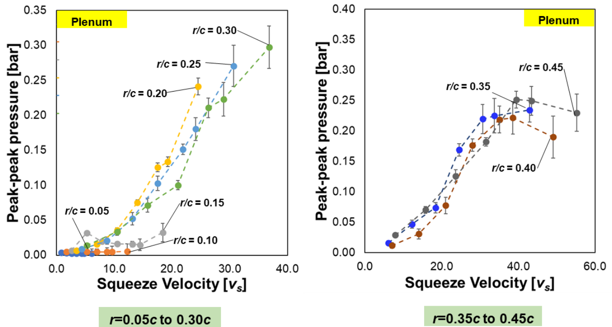
Figure 30. Peak-peak dynamic pressures in upstream plenum ( P_{pk-pk} ) vs. squeeze velocity ( v_s ). Measurements conducted at \theta=225^\circ and z=0 . CCOs with \omega = 10 Hz to 70 Hz and r = 0.05c to 0.45c .
