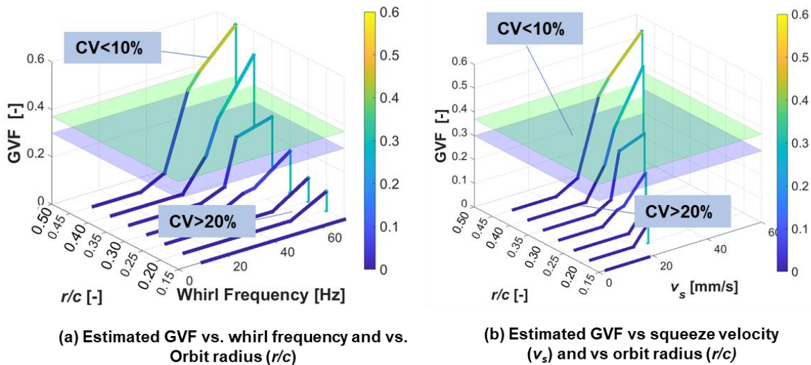
Figure 34. (a) Estimated GVF vs. orbit radius ( r/c ) and whirl frequency ( \omega ) for OR sealed SFD. (b) Estimated GVF vs. ( r/c ) and squeeze velocity ( v_s ).
