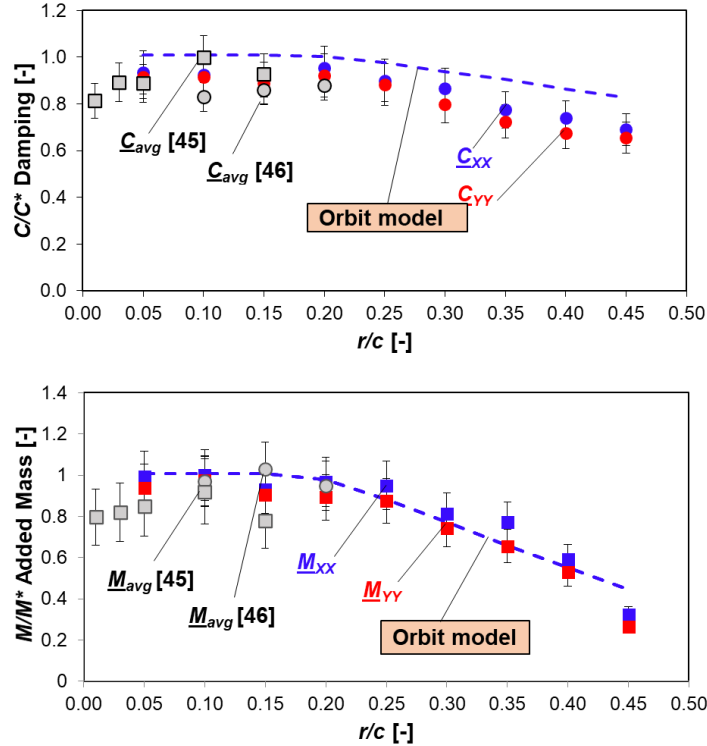
Figure 20. Normalized experimental damping ( C_{SFD} ) and inertia ( M_{SFD} ) coefficients vs. orbit radius ( r/c ). P_s = 0.69 bar(g). Experiments from CCOs and frequency range \omega = 10 - 40 Hz. Comparison with experimental results in Refs. [45, 46] and results from predictive model in Ref. [47]
