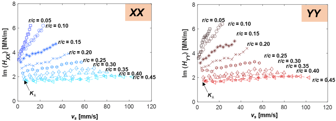
(b) \text{Im}(H_{OR})_{XX,YY} vs. squeeze velocity ( v_s ) and orbit radius ( r/c )
