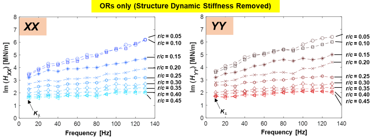
(a) \text{Im}(H_{OR})_{XX,YY} vs. whirl frequency ( \omega ) and orbit radius ( r/c )
