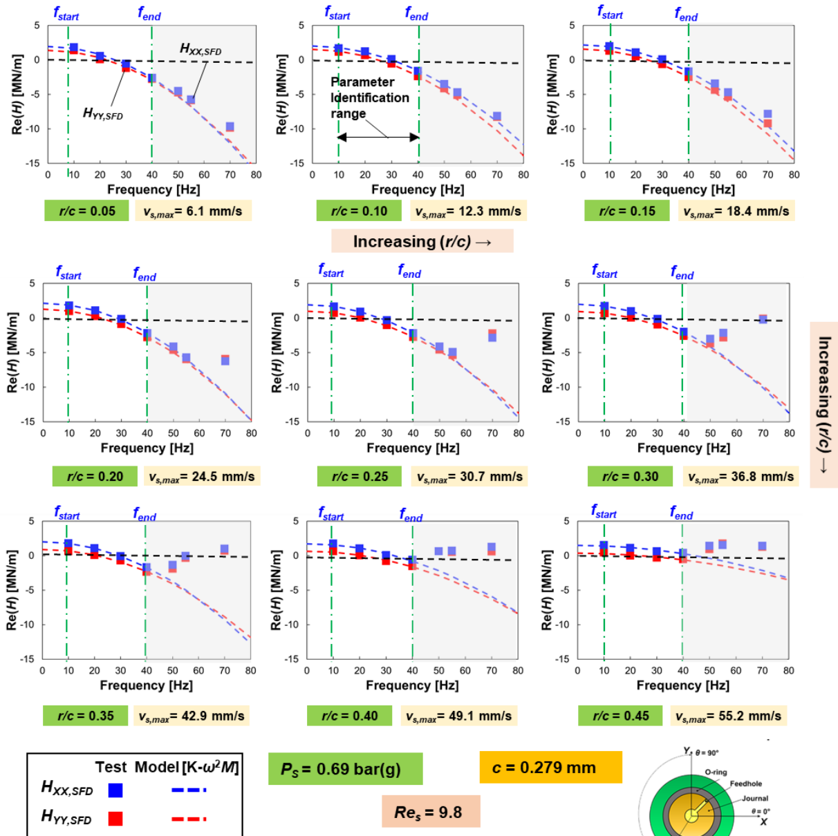
Figure 16. Real part of SFD ( H_{SFD} ) XX,YY vs. whirl frequency ( \omega ) for nine ( r/c = 0.05 to 0.45 ) CCOs. P_s = 0.69 \text{ bar(g)} . Identification of parameters ( K, M ) SFD from \omega = 10 - 40 \text{ Hz} .
