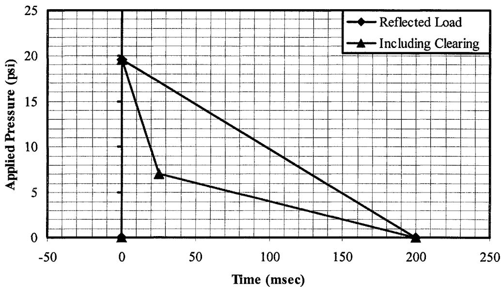
Figure 2. Effects of Clearing on Reflected Wall Load
