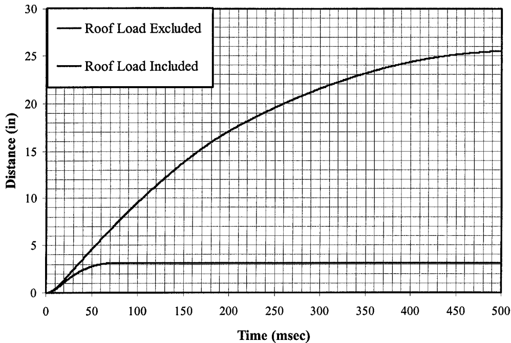
Figure 5. BRPB Sliding Response, Comparison of Effects of Roof Loading
