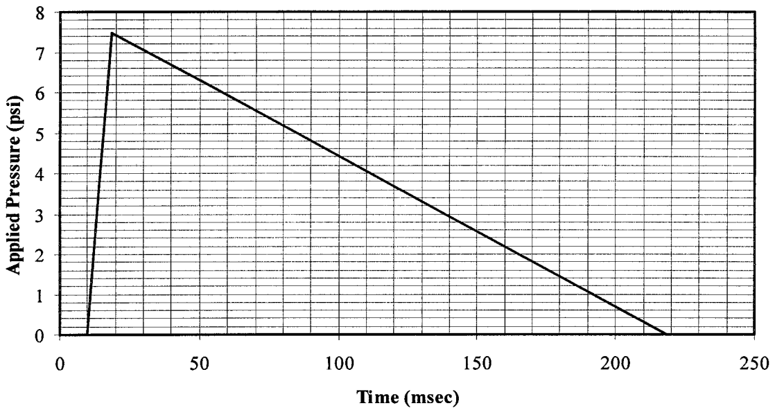
Figure 4. Back Wall Load for 8 psi free-field 200 msec Blast
