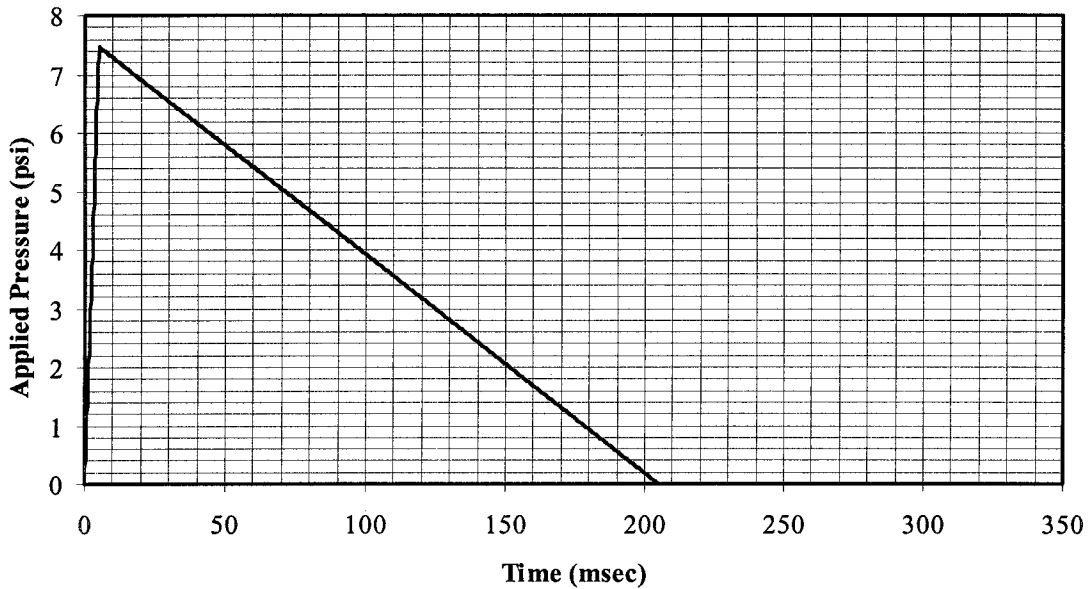
Figure 3. Roof Load for 8 psi free-field 200 msec Blast
