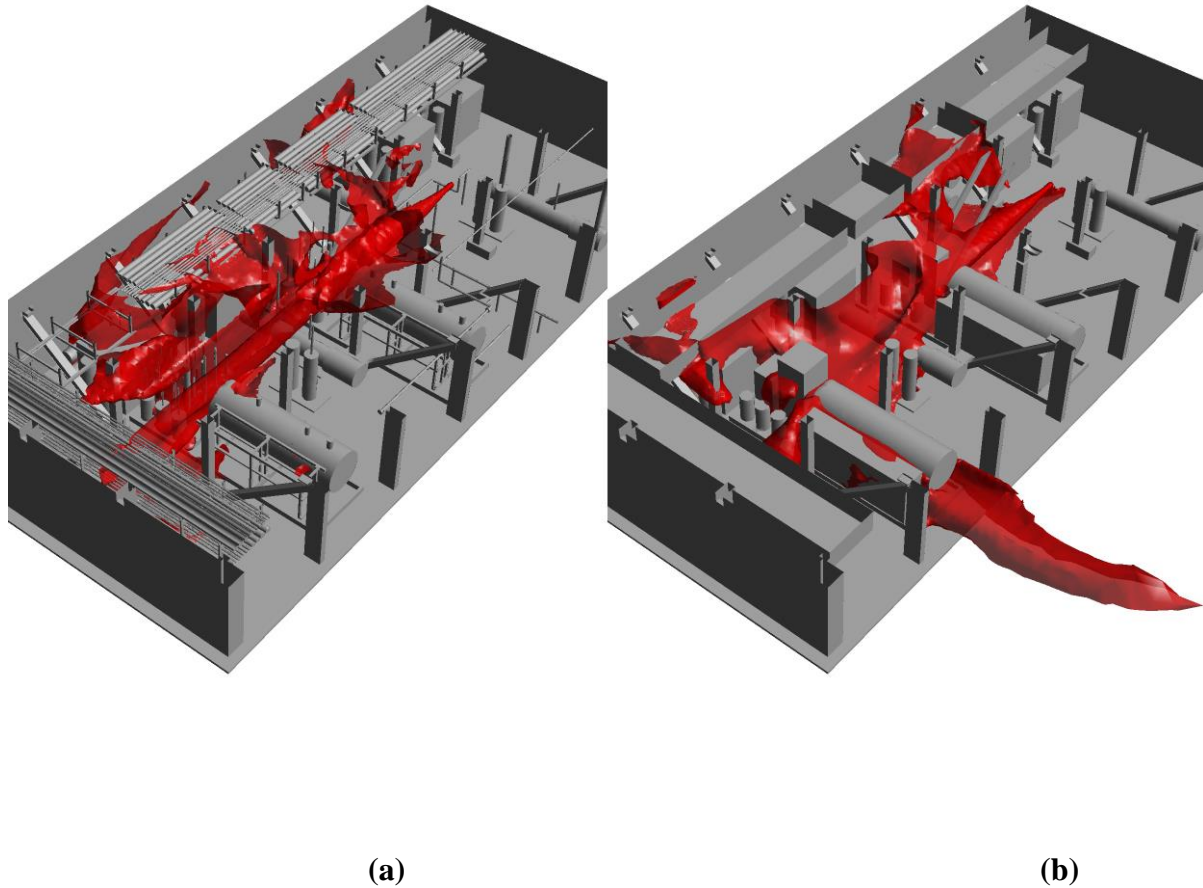
Figure 3: Iso-surface of natural gas mass fractions in (a) mesh with resolved small-scale objects and (b) mesh with small-scale objects represented using porous regions.
