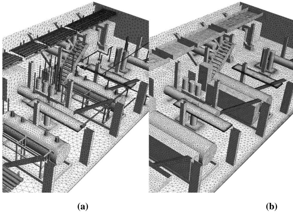
Figure 1: Surface mesh used for (a) geometry with resolved small-scale objects and (b) mesh with small-scale objects represented using porous regions. Mesh for test 16 is shown in this figure.
