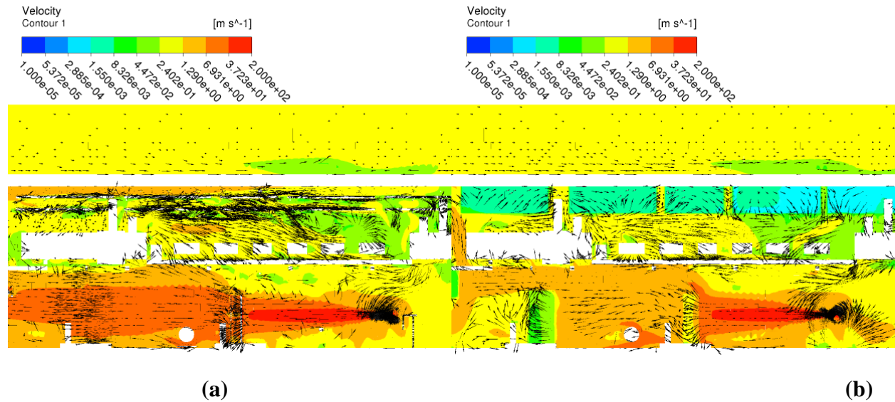
Figure 2: Contour plots of velocity magnitude (a) mesh with resolved small-scale objects and (b) mesh with small-scale objects represented using porous regions
