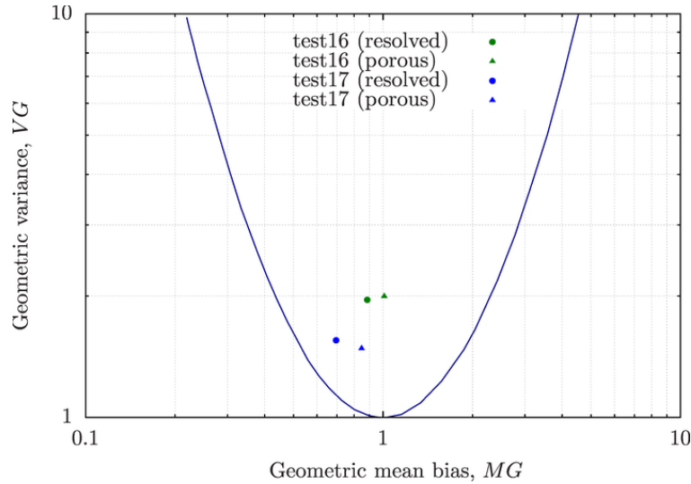
Figure 5: Geometric mean and variance showing the performance of the 4 simulations with experimental measurements.
