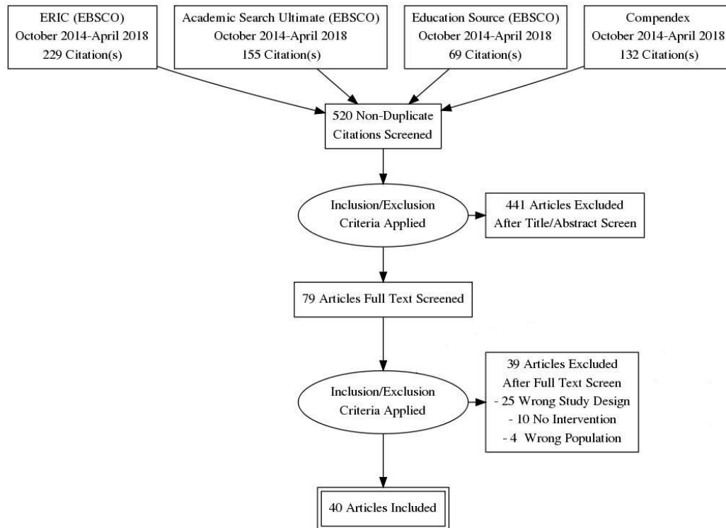
Figure 1. PRISMA flowchart
