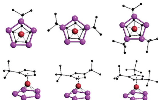
Fig. 5 Solid state structures of the complexes [ \text{Cp}^\text{R}\text{Fe}(\eta^5\text{-P}_5) ] 6a (left), [ \text{Cp}^\text{R}\text{Fe}(\eta^5\text{-P}_5) ] 6b (middle), [ \text{Cp}^\text{R}\text{Fe}(\eta^5\text{-P}_5) ] 6c (right); (top) viewing direction perpendicular to the \text{P}_5 plane revealing a nearly eclipsed arrangement of the Cp rings to the \text{P}_5 rings for all three complexes. (Bottom) side view of the complexes 6a-c .
