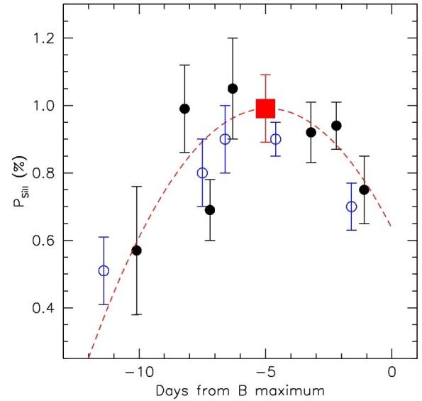
Fig. 26. Linear polarization of Si II 6355Å as a function of epoch. The dashed line is a second order polynomial fitting to SN 2006X data and the filled square dot is the polarization interpolated for day -5 (see Sect. 6.1). The empty circles are the data for SN 2002bo (Wang et al. 2007).
