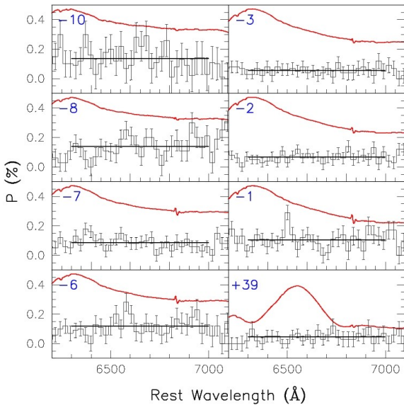
Fig. 25. Polarimetric evolution of the 6200-7000Å continuum. The smooth solid curve traces the unbinned flux spectrum, arbitrarily scaled for presentation. The horizontal line is placed at the average polarization level within the wavelength range 6300-7000Å.
