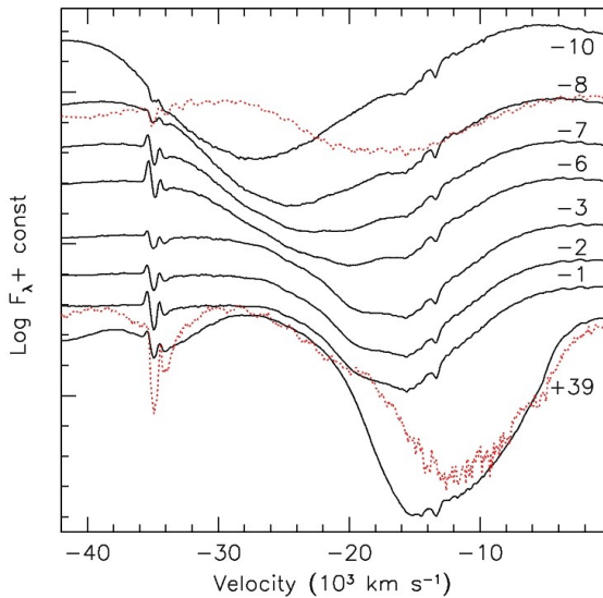
Fig. 4. Evolution of the Ca II IR triplet velocity profile. Velocities are relative to the gf -values weighted average triplet wavelength ( 8567\text{\AA} ). The dotted, light-colored curves are the spectra of SN 2002bo (Benetti et al. 2004) at 8.5 days before maximum (top) and 39.9 days after maximum light (bottom).
