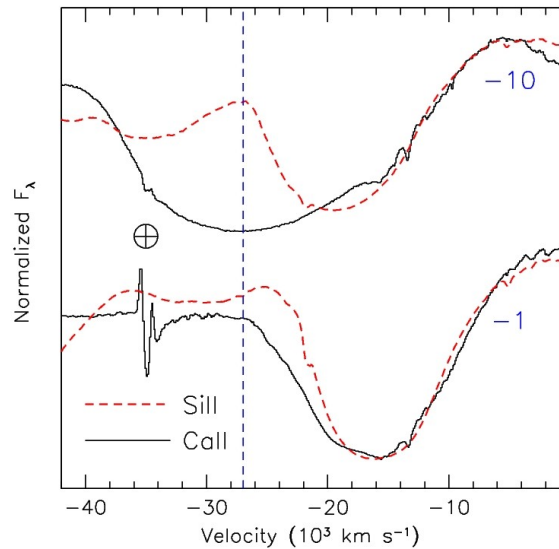
Fig. 5. Si II and Ca II line profiles on day -10 (top) and -1 (bottom). The vertical dashed line marks the Si II cutoff velocity for day -10 .
