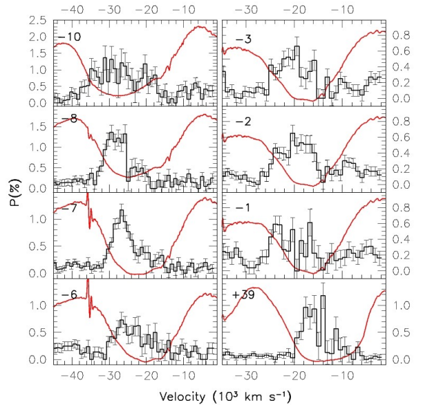
Fig. 16. Polarimetric evolution of the Ca II IR triplet profile. The smooth solid curve traces the unbinned flux spectrum, arbitrarily scaled for presentation. Note the different vertical and horizontal scales in each plot.
