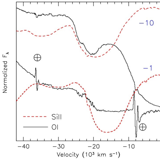
Fig. 22. O I 7774Å and Si II 6355Å line profiles on days -10 (top) and -1 (bottom).
