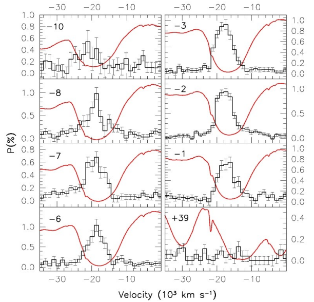
Fig. 12. Polarimetric evolution of the Si II 6355Å line profile. The smooth solid curve traces the unbinned flux spectrum, arbitrarily scaled for presentation. Note the different vertical scales in each plot. The weak feature around -22,000 \text{ km s}^{-1} is due to IS Na I D absorption.
