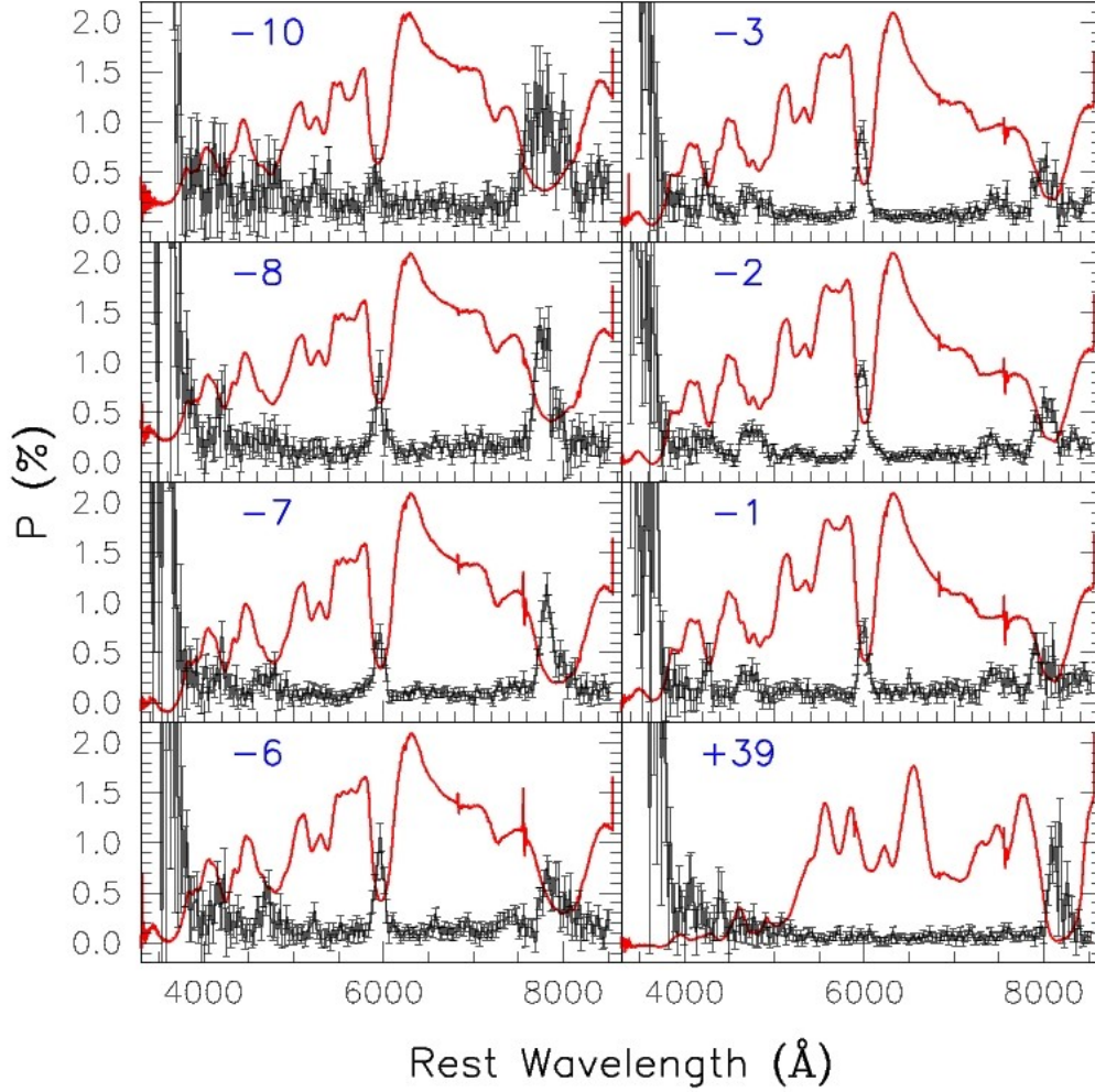
Fig. 9. Spectropolarimetric evolution of SN 2006X. For each epoch the ISP-corrected polarization degree is presented together with the unboxed flux spectrum (solid line). Epochs refer to B maximum light.
