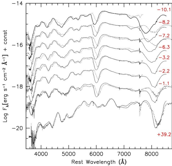
Fig. 2. Spectral evolution of SN 2006X. Phases refer to B maximum light (JD=2,453,786.17; Wang et al. 2008a). For comparison, the spectra of SN 2002bo (Benetti et al. 2004) are also plotted (dotted lines). For presentation, the observed spectra of SN 2002bo (not corrected for extinction) were reddened using a standard extinction law ( R_V=3.1 ) and E_{B-V}=0.8 .
