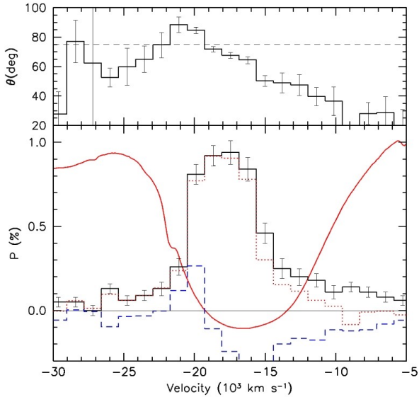
Fig. 14. Same as Fig. 13 for day -2 . The horizontal dashed line in the upper panel indicates the dominant axis deduced on day -7 .
