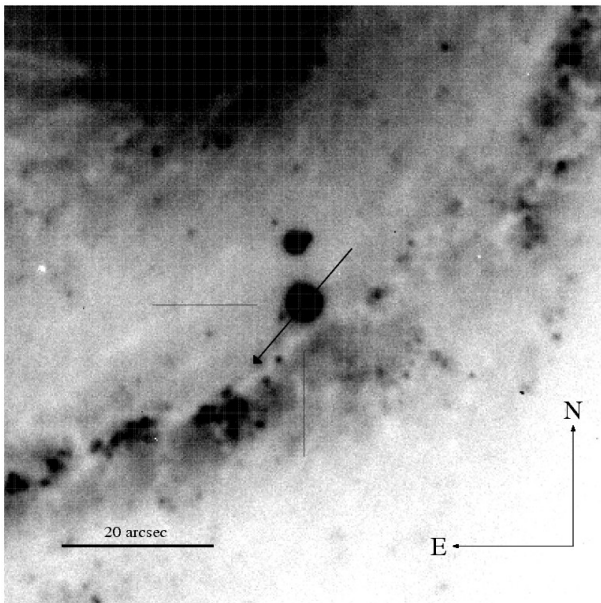
Fig. 1. SN 2006X in NGC 4321. The R band image was obtained with VLT-FORS1 (see Sect. 2) on February 11, 2006 (30 sec exposure time). The arrow placed at the SN position indicates the inter-stellar polarization position angle (139.5 degrees; see Sect. 4).
