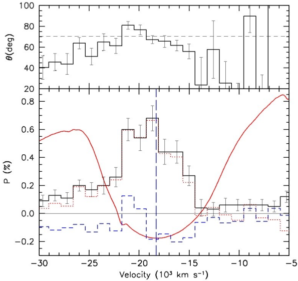
Fig. 13. Lower panel: polarization profile of Si II 6355Å on day -7 . Dotted and dashed lines trace P_d and P_o respectively (see Sect. 5.1). The vertical dashed line indicates the expansion velocity deduced from Si II 6355Å absorption minimum for this epoch. Upper panel: polarization position angle. The horizontal dashed line indicates the average angle computed in the velocity range -23,000 \leq v \leq -17,000 \text{ km s}^{-1} . The weak absorption feature around -22,000 \text{ km s}^{-1} is due to IS Na I D.
