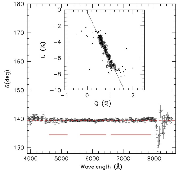
Fig. 8. Linear polarization position angle for the last epoch. The dashed line is placed at the average value computed within the wavelength ranges indicated by the three horizontal segments. The insert shows the observed Q - U plane. Circles mark data within the selected wavelength ranges, while the straight line is a best fit to this data subset.
