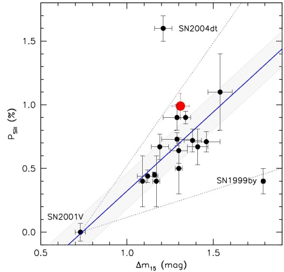
Fig. 27. Degree of polarization across the Si II 6355Å line as a function of light curve decline rate. Data are from Wang et al. (2007). SN 2006X is marked by the large dot. The solid line is a best fit to all data, with the exception of SN 1999by and SN 2004dt. The dotted lines trace the 1- \sigma level of the intrinsic polarization distribution generated by the Monte-Carlo simulation discussed by Wang et al. (2007). The shaded area indicates the rms deviation of the data points from the best fit relation.
