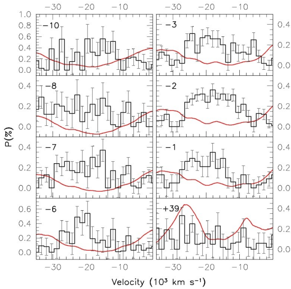
Fig. 24. Polarimetric evolution of the Si II 5051Å line profile. The smooth solid curve traces the unbinned flux spectrum, arbitrarily scaled for presentation.
