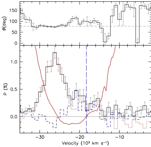
Fig. 17. Lower panel: polarization profile of Ca II IR triplet on day -7 . Dotted and dashed lines trace P_d and P_o respectively (see Sect. 5.1). The vertical long-dashed line indicates the expansion velocity deduced from the Si II 6355Å line at the same epoch. Upper panel: polarization position angle. The horizontal dashed line indicates the average angle computed in the velocity range -30,000 \leq v \leq -24,000 \text{ km s}^{-1} . The feature around -15,000 \text{ km s}^{-1} is due to a telluric absorption.
