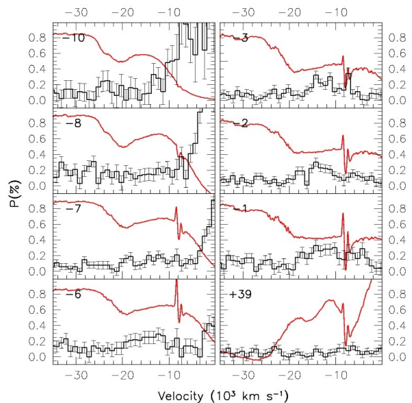
Fig. 21. Polarimetric evolution of the O I 7774Å line profile. The smooth solid curve traces the unbinning flux spectrum, arbitrarily scaled for presentation. The broad polarized feature on the right edge is the blue wing of the Ca II near-IR triplet.
