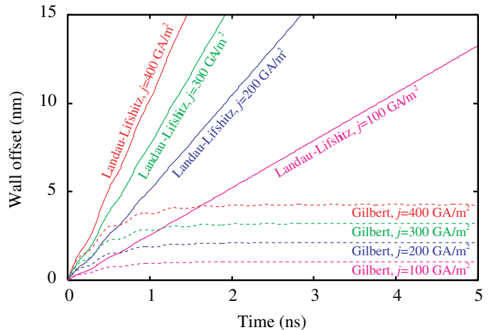
FIG. 1: Position versus time for a transverse domain wall and several values of the applied current density computed with adiabatic spin torques ( \beta = 0 ) and the two forms of damping in (4) and (5).
