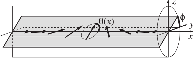
FIG. 2: A one-dimensional Néel domain wall with magnetization \mathbf{M}(x) .
