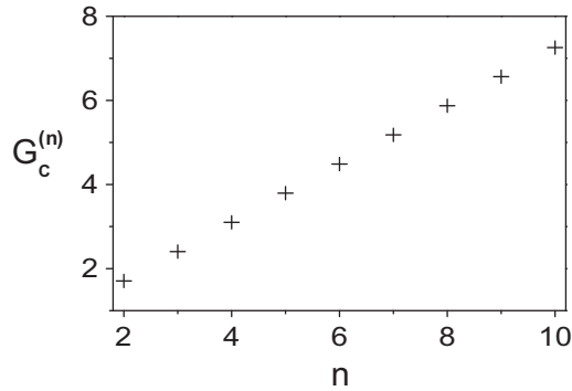
Figure 1. Critical gain G_c^{(n)} at which the nonclassicality condition \text{Det}[M^{(n)}] < 0 ceases to be valid for the one-photon Fock state under PILA.
