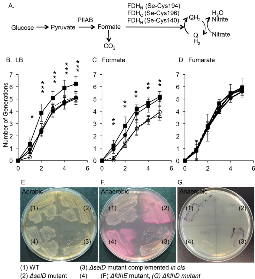
FIG 6 The \Delta selD ( \Delta STM1297 ) mutant is defective in anaerobic growth in the presence of formate. (A) Overview of formate metabolism in Salmonella Typhimurium . Q, ubiquinone; QH 2 , ubiquinol. (B to D) The inability to metabolize formate results in growth defect under anaerobic conditions. Overnight cultures of the wild type (filled squares), \Delta selD (open circles), \Delta selD strain complemented in cis (filled circles), and \Delta fdhD (open triangles) were subcultured in LB broth (B), LB broth supplemented with 40 mM formate (C), or 40 mM fumarate (D) and grown in an anaerobic chamber at 37°C. Aliquots were collected hourly (the times [in hours] are indicated on the x axis), serially diluted, and plated for CFU enumeration. Each data point represents the mean number of generations calculated as described in Materials and Methods and standard deviations of at least three independent experiments. Statistical significance was determined by t test. *, P < 0.05 (statistically significant difference in growth of mutant strains compared to wild type); multiple asterisks, more than one mutant strain is significantly different from wild type. (E to G) The \Delta selD mutant accumulates formate during growth on MacConkey nitrate agar due to the loss of active formate dehydrogenases (FDH N ) under anaerobic conditions (F) but not under aerobic conditions (E). (G) When the \Delta selD mutant is grown anaerobically, it did not display formate dehydrogenase (FDH H ) activity using the benzyl viologen overlay assay.
