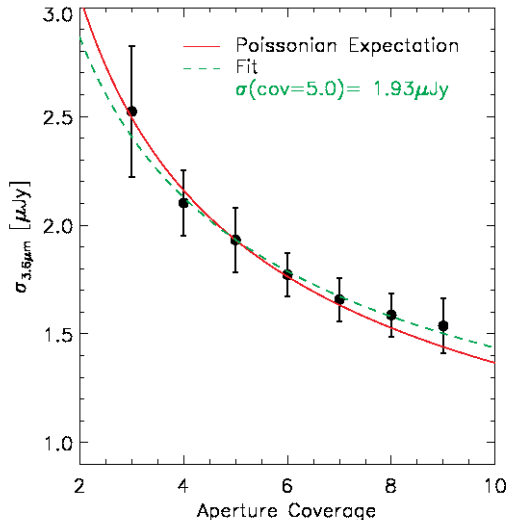
Fig. 4.— Sky background noise, \sigma , as a function of aperture coverage (see text for details). The expected trend for background-dominated noise is shown with a red solid line, while the observed best fit relation is shown with a green dashed line. We cut the IRAC 3.6 \mu\text{m} catalog at a 3\sigma level, where \sigma is estimated from the average coverage of each source.
