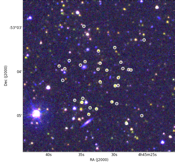
Fig. 13.— False color image (red= 4.5\ \mu\text{m} , green= 3.6\ \mu\text{m} , and blue= R_c ) showing a 3'7 \times 3'7 region around one of the galaxy cluster identified in the central square degree where optical data are available. Open circles show galaxies with red 3.6\text{--}4.5\ \mu\text{m} color, 3.6\ \mu\text{m} and R_c magnitudes fainter than 18.7 and 21, respectively.
