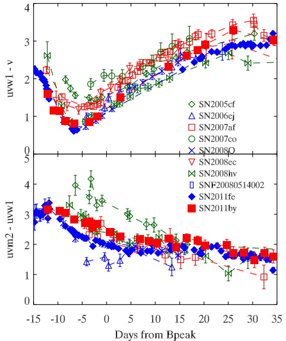
FIG. 2.— Color curves of SNe 2011by and 2011fe along with other young, normal SNe Ia (Brown et al. 2014b). The uvw1-v colors of SNe 2011by and 2011fe are very similar. The uvm2-uvw1 colors of SNe 2011by and 2011fe are distinct (but small) at all times, but the difference becomes smaller with time.
