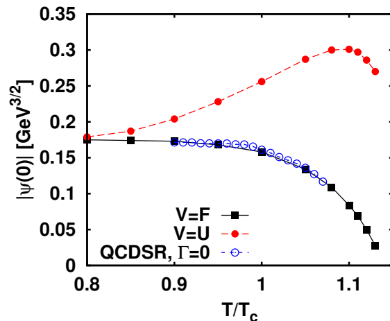
FIG. 3: (Color online) Temperature dependence of |\psi(0)| obtained from the free energy (filled squares) and internal energy (filled circles) potentials together with that from the QCD sum rule (open circles).
