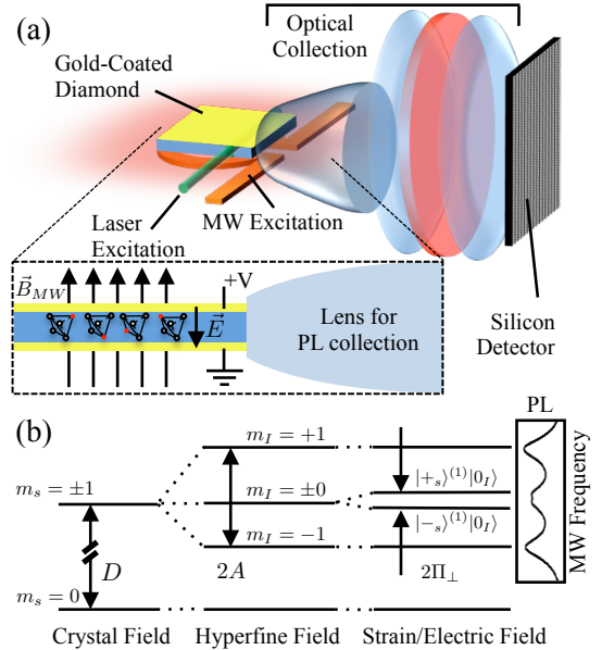
FIG. 1. (a) Diamond electrometry setup. For applying electric fields across the ensemble of NV - s, gold electrodes were evaporated on both faces of the diamond plate (3 x 3 x 0.32 mm 3 ). A collimated laser beam ( \sim 200 \mu\text{m} diameter) was used to excite a single pass of NV - s input from the edge of the diamond plate, and microwave (MW) excitation was delivered to the ensemble of NV - s by a stripline in an ‘ \Omega ’ shape patterned on a printed circuit board. Inset A cross-section of the experiment depicting four of the eight total NV - orientations within an ensemble of NV - s used for detecting electric fields. (b) Generalized diagram depicting how crystal ( D ), hyperfine ( A ), strain and the magnitude of transverse electric fields ( \Pi_{\perp} = \sqrt{\Pi_x^2 + \Pi_y^2} ) affect energy splitting in both the ground- and excited-state spin configurations of the NV - . The spin labels ( m_s and m_I ) indicate the quantum numbers of the electronic and hyperfine states, and the two eigenstates that are sensitive to electric fields are given by: |+\rangle_s^{(1)}|0\rangle_I ( m_I = +0 ) and |-\rangle_s^{(1)}|0\rangle_I ( m_I = -0 ). The inset to the right shows the ground-state ODMR spectra of an ensemble of NV - s.
