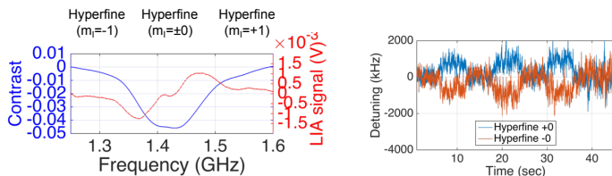
FIG. 6. Excited-state ODMR spectra measured on an NV^- ensemble at zero magnetic field. Excited-state shifts due to pulsed electric fields applied to an NV^- ensemble at zero magnetic field. The sensitivity of this measurement approaches 300 \frac{V/cm}{\sqrt{Hz}} .
