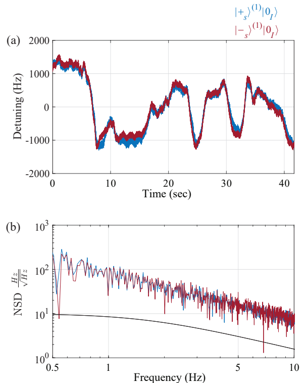
FIG. 3. Measurements taken at 1.8 W laser excitation with a high-stability bias voltage of 225 Volt. (a) Time trace of both lock-in-amplifier channels monitoring frequency detuning of ensemble states |+\rangle_s^{(1)}|0\rangle_I (blue) and |-\rangle_s^{(1)}|0\rangle_I (red) in units of transition frequency noise per \sqrt{\text{Hz}} . (b) Noise spectral density (NSD) of both channels. The noise floor of the red (blue) channel is calculated to be equivalent to 12.6 \pm 6.4 ( 13.4 \pm 7.4 ) V/cm/ \sqrt{\text{Hz}} , assuming the noise is entirely attributed to electric field fluctuations. The electric field sensitivity estimated by the shot-noise limit is given by the black line ( 1.2 \pm 0.1 V/cm/ \sqrt{\text{Hz}} ).
