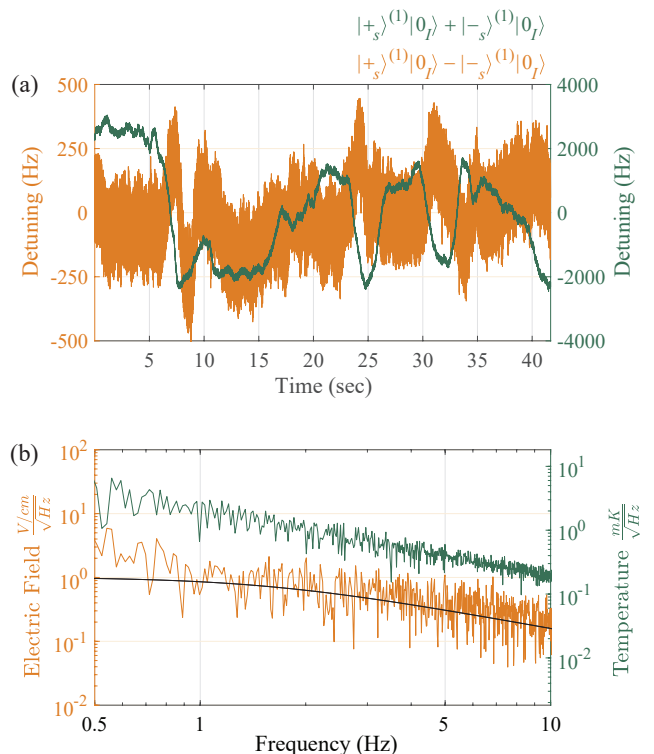
FIG. 4. Identical experimental measurements as in Fig. 3 except the analysis takes advantage of the experimental methodology for deconvolving fluctuations from temperature and electric fields. (a) Time trace of the difference (orange, electric field) and sum (green, temperature) of the lock-in-amplifier channels from Fig. 3. (b) NSD on the time-trace difference (sum) of the two channels, which corresponds to a sensitivity of 1.6 \pm 1.2 \text{ V/cm}/\sqrt{\text{Hz}} ( 2.4 \pm 1.2 \text{ mK}/\sqrt{\text{Hz}} ) due the transverse electric field (temperature) fluctuations. The sum of the two correlated channels yields a shot-noise sensitivity limit of 0.9 \pm 0.1 \text{ V/cm}/\sqrt{\text{Hz}} (black line), which is \sqrt{2} times lower than that of the individual channels as seen in Fig. 3b.
