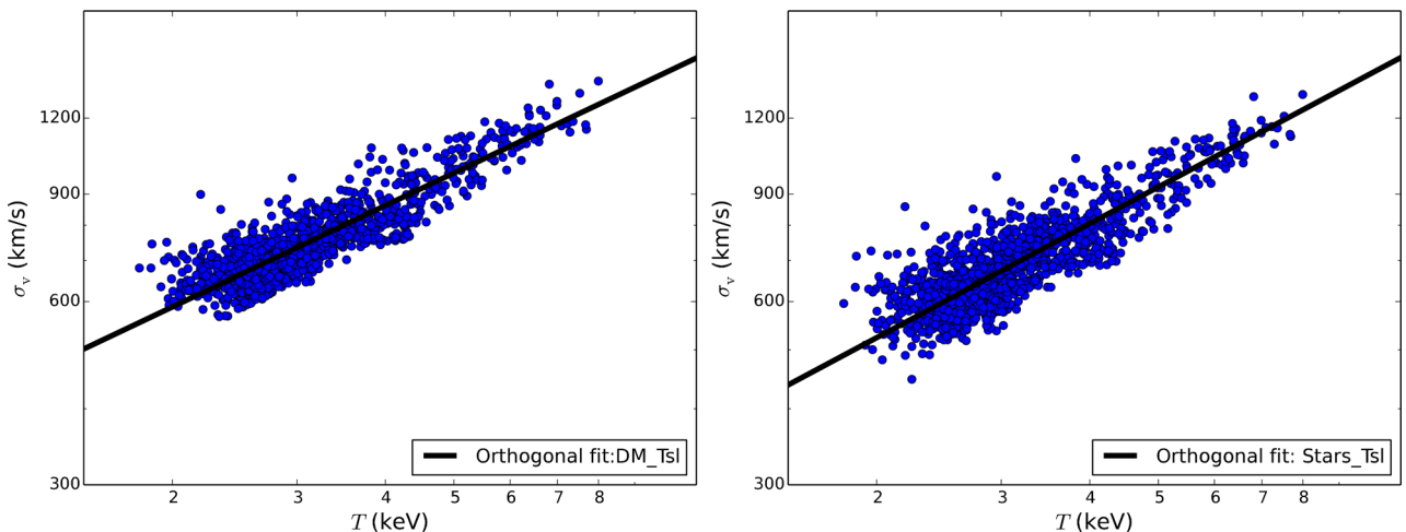
Figure 8. The \sigma_v-T relation for the Millennium Gas Project simulations using dark matter and stars as proxies for the velocity dispersion. The blue dots are the data obtained from the simulation and the solid black line shows the fit using the orthogonal regression method. The slope is slightly steeper for the stars ( B = 0.62 \pm 0.01 ) than for the dark matter ( B = 0.55 \pm 0.08 ) but both are consistent with previous studies of the \sigma_v-T relation and the results obtained from our data.
