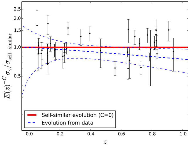
Figure 7. Plot showing the evolution of the normalization of the \sigma_v-T relation obtained for the data with the 95 percent confidence intervals in the dashed lines as compared to the self-similar relation which predicts no evolution shown as the solid line. The black points show our sample data.
