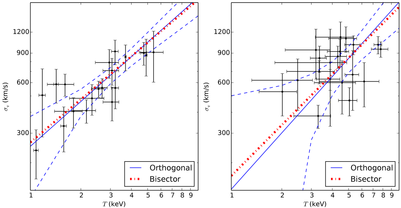
Figure 3. The \sigma_v - T relation assuming no evolution, i.e. C = 0 in equation (3), for low (left -0.0 < z < 0.5 ) and high (right -0.5 < z < 0.9 ) redshift samples. The solid blue line shows an orthogonal regression fit to the data with the dashed line representing the 95 per cent confidence interval. The dot-dashed line shows a bisector regression fit to the data (see Section 3.2). A model of the form seen in equation (3) was used in the Metropolis algorithm to determine a line of best fit (see Section 4.1). It is interesting to note that the two best-measured systems (XMMXCS J105659.5-033728.0 and XMMXCS J114023.0+660819.0) in the high-redshift subsample are relatively far off the best-fitting relation, with a higher than predicted temperature. Our current observations do not provide good enough spatial resolution or deep enough multicolour photometry to determine the exact reason for this and require further study and re-observations.
