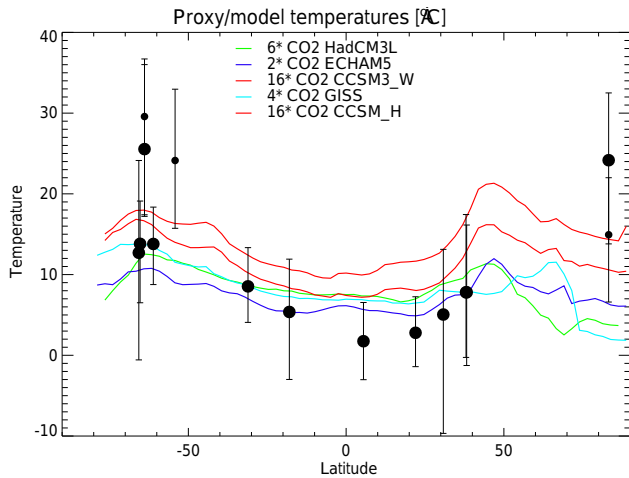
Figure 1. Zonal mean Eocene sea-surface temperature warming, presented as an anomaly relative to present or pre-industrial values. Warming from the five models in “Eomip” (Lunt et al., 2012) are shown as coloured lines; for each model only the CO 2 concentration that best fits the temperature proxy observations is shown. Warming derived from the proxies are shown as filled circles, with error bars representing the range of uncertainty associated with proxy calibration and temporal variability. Larger symbols represent “background” early Eocene state, smaller symbols represent the EECO. Adapted from Fig. 8a in Lunt et al. (2012).
