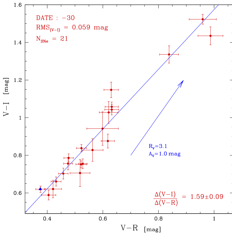
Fig. 5.— V - I versus V - R diagram for 21 SNe IIP having VRI photometry corrected for the A_G and K -terms. The blue line is a least-squares fit to the data, with a slope of 1.59 \pm 0.09 . The blue arrow has a slope of 2.12 and corresponds to the reddening vector for A_V = 1.0 \text{ mag} and a standard Galactic extinction law ( R_V = 3.1 ). The blue triangle shows the one SN of this subsample consistent with zero extinction having R -band photometry.
