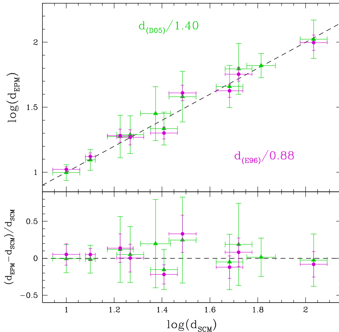
Fig. 18.— Similar to Figure 17, after removing systematic differences by bringing the EPM distances to the SCM scale (all in Mpc). Only random differences between EPM and SCM distances remain. For the E96 case the discrepancies have a spread of 16%, while for the D05 case the scatter is 13%. The dashed line in the top panel is fixed to show a slope of unity.
