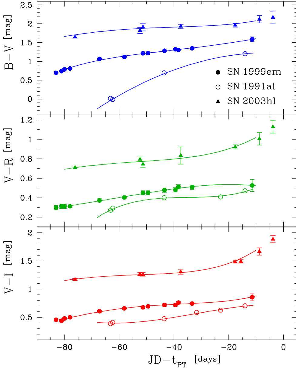
Fig. 2.— B-V , V-R , and V-I color curves of SN 1999em (filled circles), SN 1991al (open circles), and SN 2003hl (filled triangles) corrected for the A_G and K -terms. This comparison demonstrates that each SN displays a different color evolution, precluding the determination of color excesses from a simple color offset after correcting for the A_G and K -terms. For SN 1991al the error bars are always smaller than the symbols and therefore not plotted.
