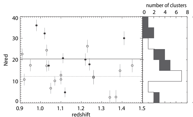
FIG. 8.— Red-sequence richness as a function of redshift. Clusters that hosted supernovae are indicated with filled symbols. Clusters that did not host supernovae are indicated with open symbols. The solid and dotted lines mark the respective median richnesses of the two samples. The histogram represents the distribution of richnesses for clusters that did not host a SN (open) and for clusters that did (filled).
