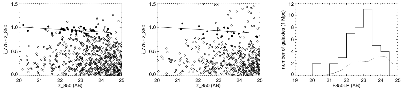
FIG. 6.— Red-sequence of WARP J1415.1+3612 compared to field galaxies from the GOODS data. (a) Left: The color magnitude diagram for galaxies in the image of WARP J1415.1+3612. (b) Center: The color magnitude-diagram for galaxies in a random GOODS field of the same area. In both color magnitude diagrams, the solid circles represent galaxies with a color and morphology expected for an early type cluster member, the open circles represent all galaxies in the image, and the solid line illustrates the modeled red-sequence at z = 1.03 . Some objects represented by open circles had colors and magnitudes near the red-sequence but did not have morphologies consistent with an elliptical galaxy. Other objects had a morphology consistent an elliptical galaxy but did not lie near the model red-sequence. (c) Right: Histogram of the red-sequence members and interlopers. The solid line represents galaxies within 0.1 mag of the red-sequence in WARP J1415.1+3612 and the dashed line represents an estimate of interlopers derived from the GOODS fields.
