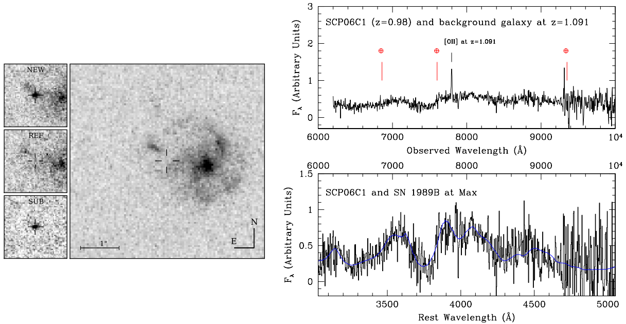
FIG. 2.— Left: The panels on the left hand side demonstrate the discovery of SN SCP06C1 from the ACS images labeled "NEW" (host galaxy with SN light), "REF" (host only), and "SUB" (residual after subtracting the reference image of the host galaxy). This SN occurred along the line-of-sight to a large background galaxy at z = 1.091 . The main panel shows the much brighter background galaxy centered west of the SN position and the potential SN host which lies NE of the SN position but does not have spectroscopic confirmation. Right/Upper Panel: The FORS2 spectrum of SN SCP06C1, a secure SN Ia at z = 0.98 . The [OII] \lambda\lambda 3727 doublet from the background galaxy can be seen in the spectrum. The spectrum is plotted in the observer frame. Strong telluric absorption features have been removed. The residuals are marked with \oplus . Right/Lower Panel: After subtracting the spectrum of the background galaxy, the spectrum is re-binned and plotted in the rest frame. The spectrum of SN 1989B at maximum light is the best matching nearby SN Ia. This SN is plotted at the blue continuous line.
