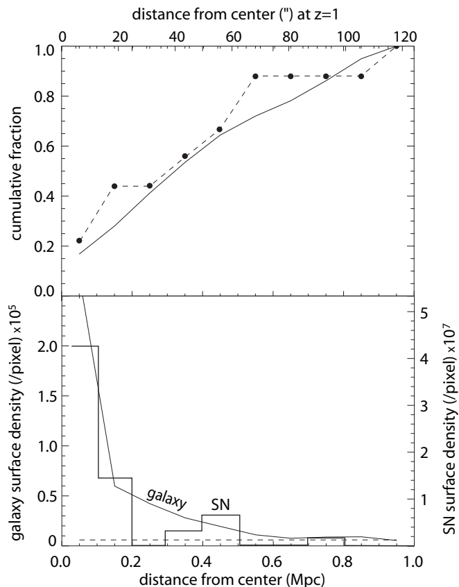
FIG. 7.— (a) Upper Panel: Cumulative distribution of red-sequence galaxies in all 25 clusters with 21 < z_{850} < 24 selected (solid line) and SNe (dashed line and solid circles). (b) Lower Panel: The solid line represents the surface density as a function of distance from the cluster center of galaxies with 21 < z_{850} < 24 selected to lie on the red-sequence for the complete sample of 25 clusters in this program. The dashed line represents the surface density of galaxies satisfying the same criteria in the GOODS data. The histogram represents the surface density of cluster SNe from this program. Because some of the cluster volume may lie outside the field, surface densities are computed from the number of pixels in the stacked ACS images within a distance r from the cluster center.
