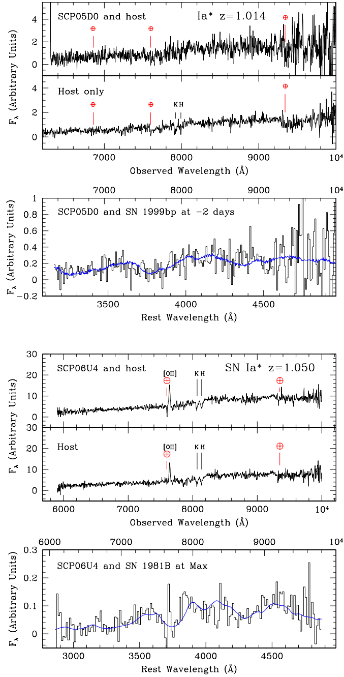
FIG. 4.— Spectra of two SNe that are heavily contaminated by the light of the host galaxy. The three panels in each plot show, from top to bottom, the spectrum of the supernova and the host, the spectrum of the host without SN light, and the host-subtracted supernova spectrum in the rest frame. The best matching nearby SNe Ia are plotted in the lowest panels in blue.
