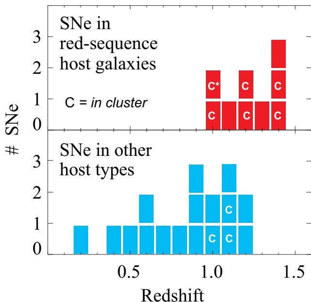
FIG. 5.— The redshift distribution of the SNe discovered in our ACS program. The upper panel shows the distribution of red-sequence galaxies that had SNe Ia, with the cluster members indicated by “C”. The asterisk indicates [OII] emission in the spectrum of a galaxy with red-sequence color and spectral features as explained in the text. The lower panel shows the distribution for the other SN hosts. For z > 0.95 , the number of SNe in cluster galaxies (9) is comparable to the number of SNe in field galaxies (7).
