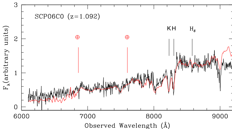
FIG. 3.— The spectrum of SN SCP06C0, an example in which the SN was considerably fainter than the host galaxy (black line). The solid red line is the spectral template of an elliptical galaxy from Kinney et al. (1990). The colors of the host of SN SCP06C0 places it within the red sequence of the cluster (see Appendix A to see how this is defined) and the spectrum is, qualitatively, a good match to the spectrum of an elliptical galaxy.
