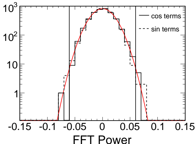
FIG. 2: The distributions for the even (cos) and the odd (sin) mean powers for harmonic frequencies to 4\omega_{\oplus}T_{\oplus} from the FFT analysis of 1,000 simulated experiments in Run I and Run II. Superposed on these distributions is a Gaussian fit of width \sigma = 1.8 \times 10^{-2} . This fit was obtained independently for both distributions. Values outside of the vertical lines are more than 3\sigma from the mean.
