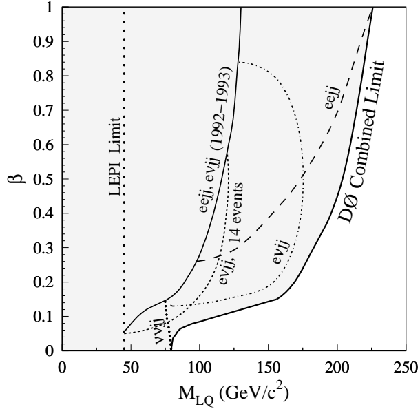
FIG. 22: The 95% C.L. lower limit on the mass of first-generation scalar leptoquarks as a function of \beta for the individual eejj , e\nu jj , and \nu\nu jj channels, and for the combined analysis.
