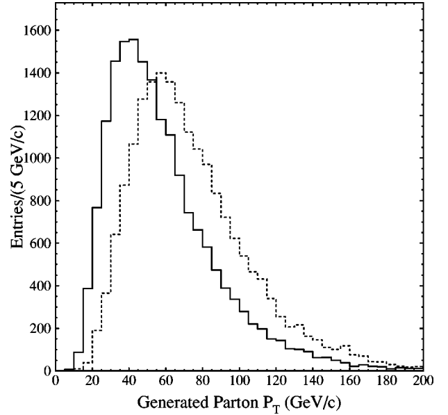
FIG. 9. P_T distributions for partons from top quark decays obtained from the HERWIG Monte Carlo program after simulation of detector response and including the effects of the top quark mass candidate sample data selection. The solid line indicates the distribution for light quarks from the W \rightarrow q\bar{q}' decay and the dashed line is the distribution for b quarks.
