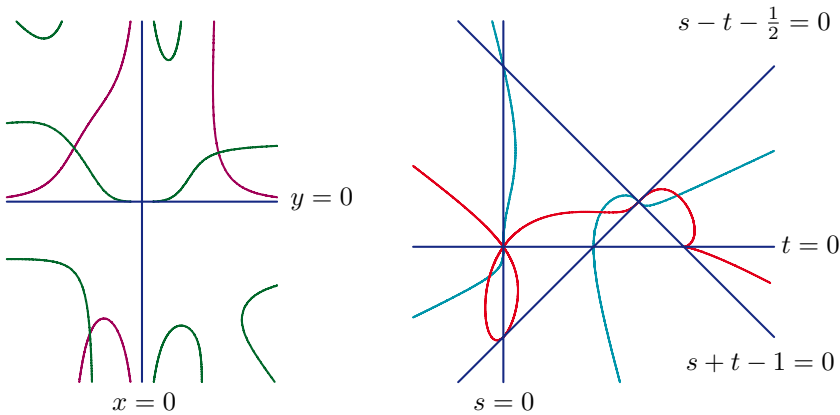
Figure 2.1. The polynomial system (2.4) and the system of master functions (2.5).
