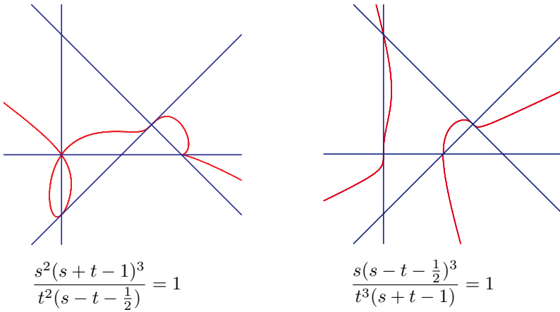
Figure 1.1. Master function curves.
